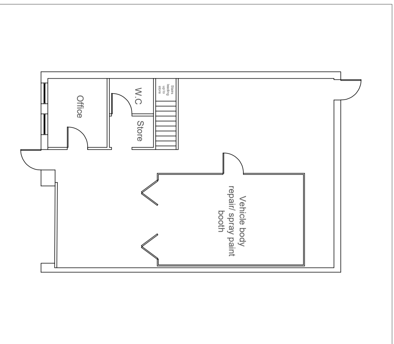
Floor-plan Proposed Scale 1/100
