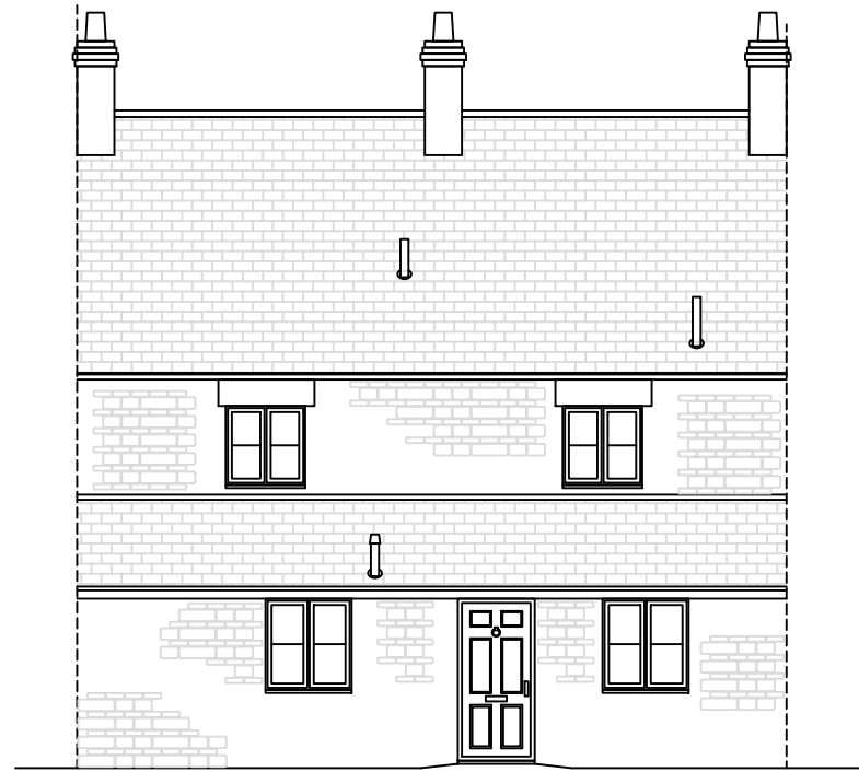
FRONT ELEVATION
