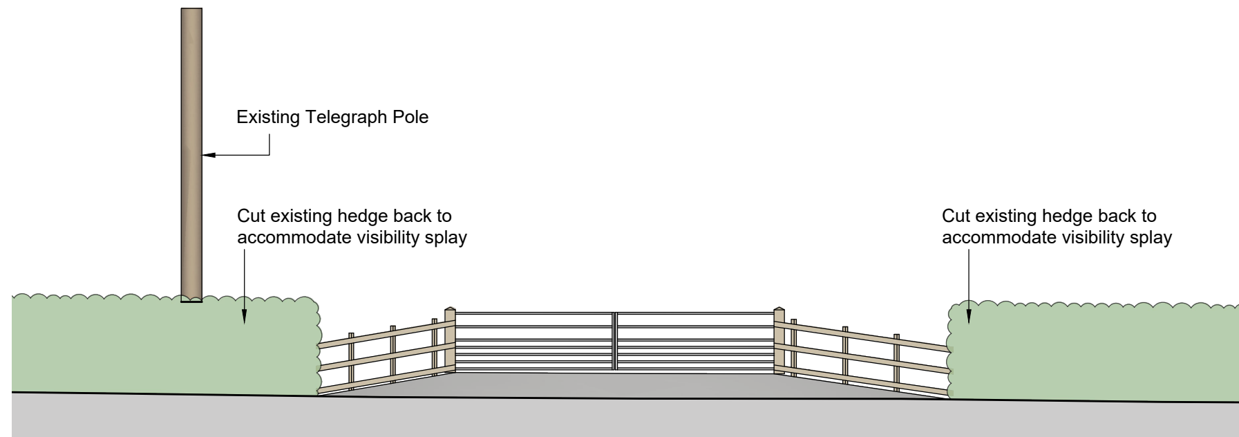
PROPOSED ELEVATION
