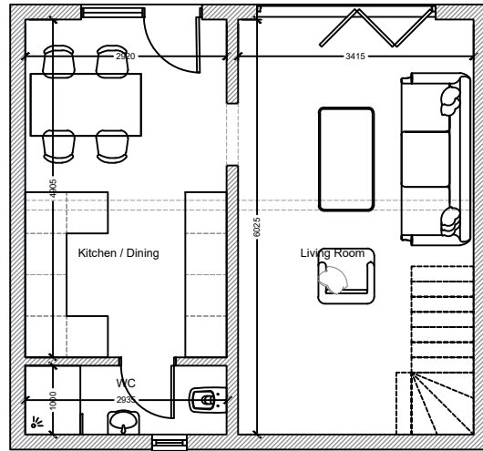
EXISTING FLOOR PLAN SCALE - 1:100 @ A3
