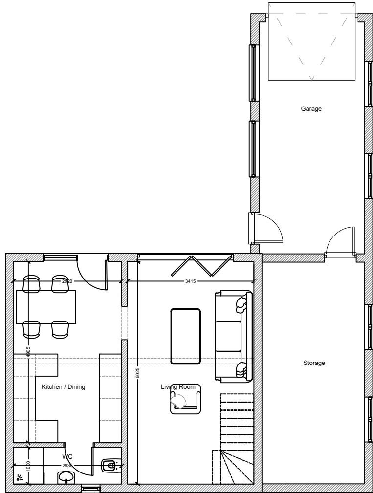
PROPOSED FLOOR PLAN SCALE - 1:100 @ A3
