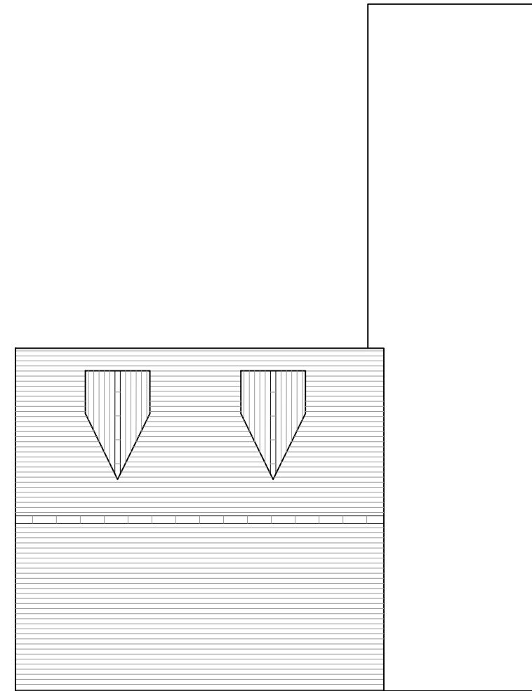
PROPOSED ROOF PLAN SCALE - 1:100 @ A3
