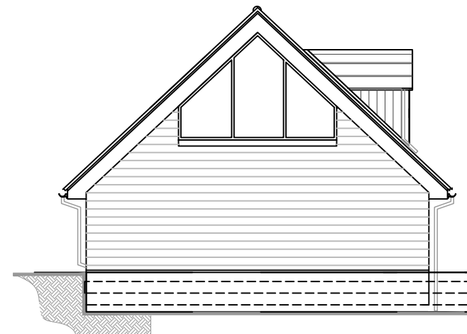
EXISTING NORTH ELEVATION SCALE - 1:100 @ A3
