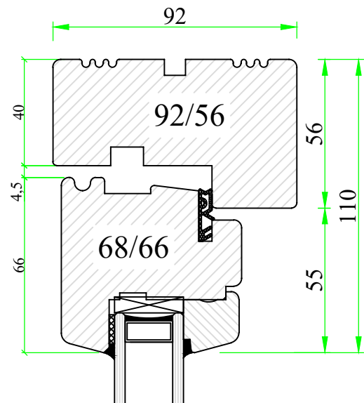
Frame Head
