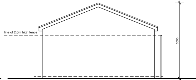
East Elevation
