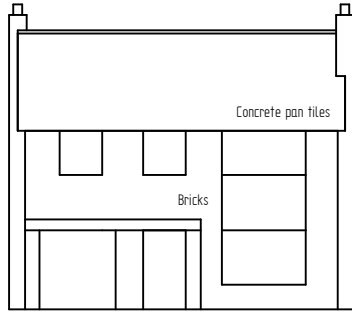
Existing Front 1:100
