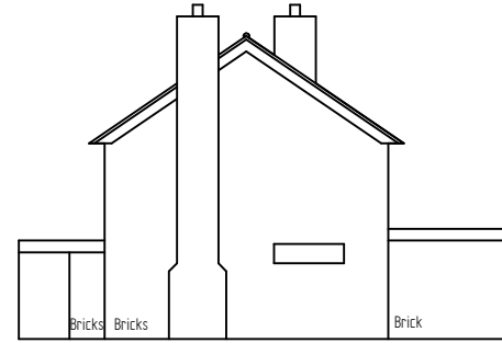
Existing Side 1:100
