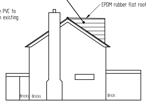
Proposed Side 1:100
