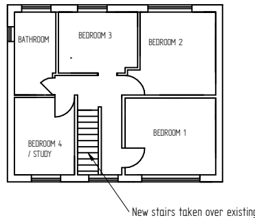
Proposed First Floor 1:100
