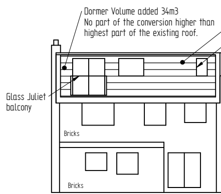
Proposed Rear 1:100
