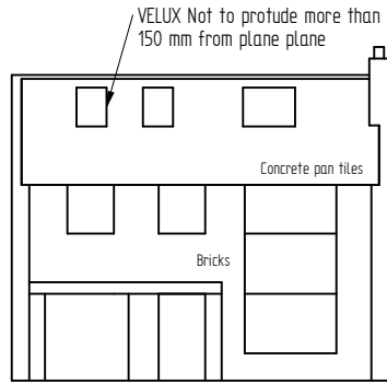
Proposed Front 1:100
