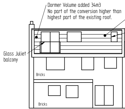
Proposed Rear 1:100
