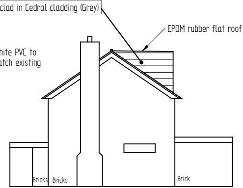
Proposed Side 1:100
