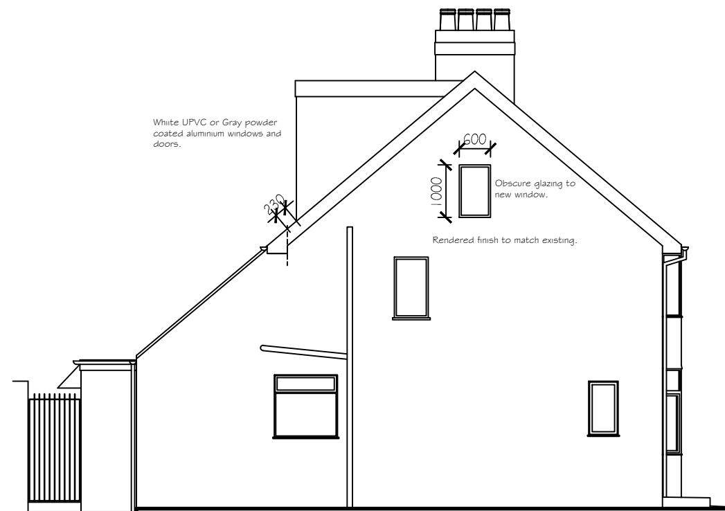
Side Proposed Elevations
