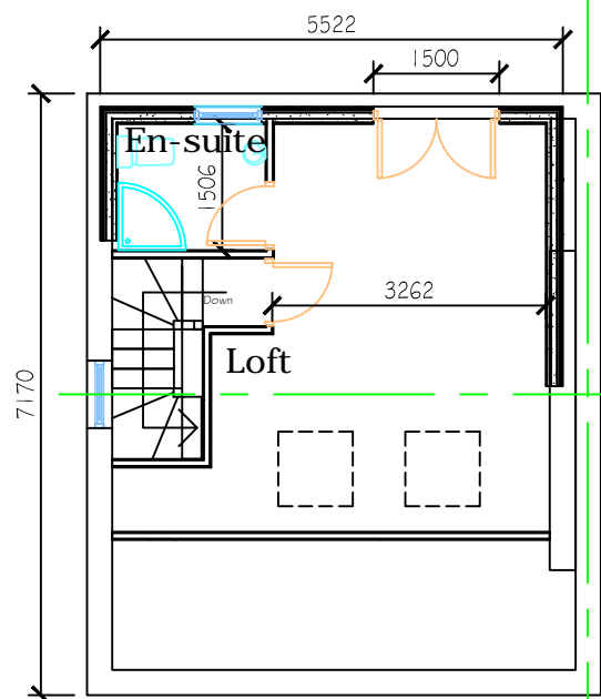
Loft Proposed Plans
