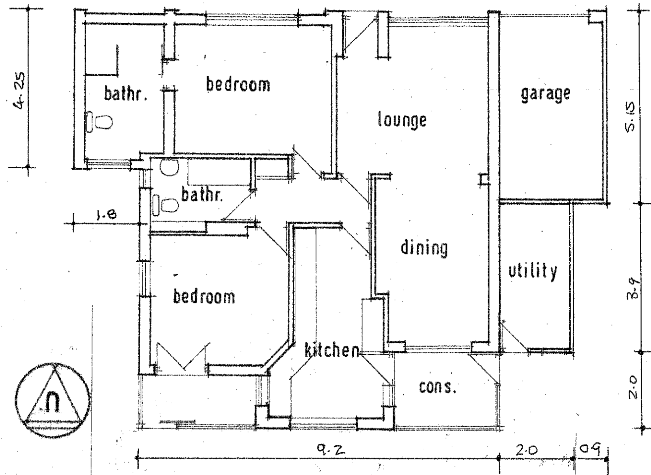
existing plan
