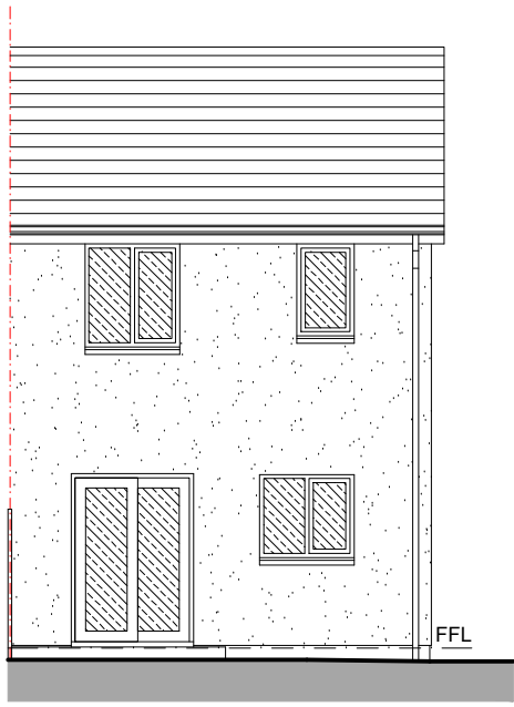
REAR ELEVATION (1:100)
