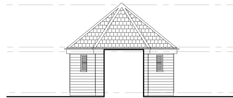
SIDE ELEVATION PROPOSED 1:100 @ A1
