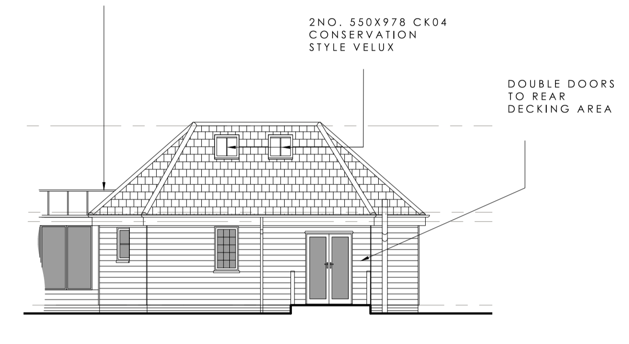
REAR ELEVATION PROPOSED 1:100 @ A1
