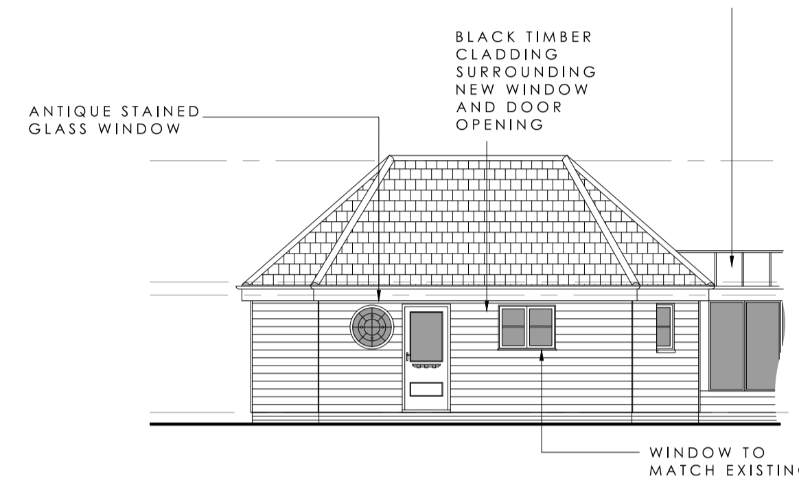
FRONT ELEVATION PROPOSED 1:100 @ A1
