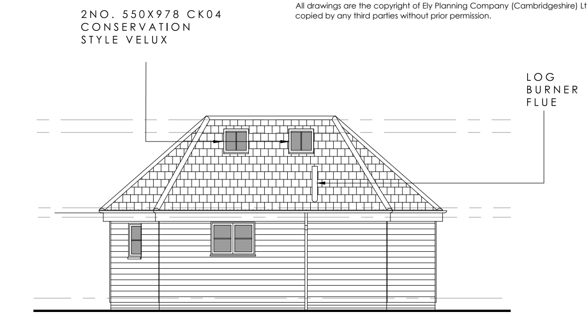
REAR ELEVATION PROPOSED 1:100 @ A1
