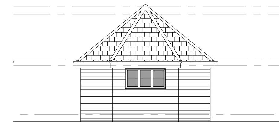
SIDE ELEVATION PROPOSED 1:100 @ A1
