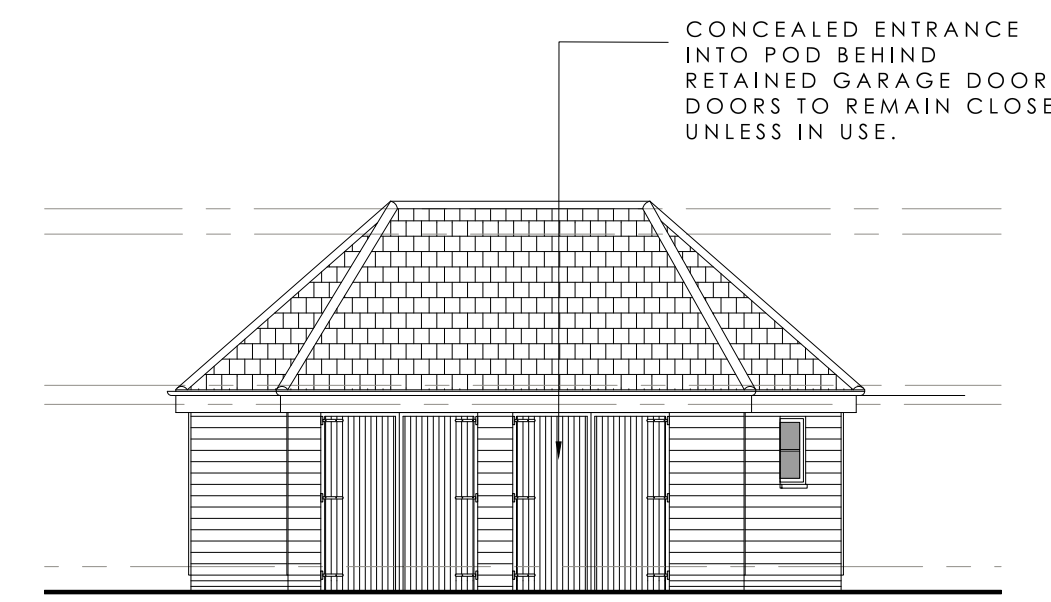
FRONT ELEVATION PROPOSED 1:100 @ A1
