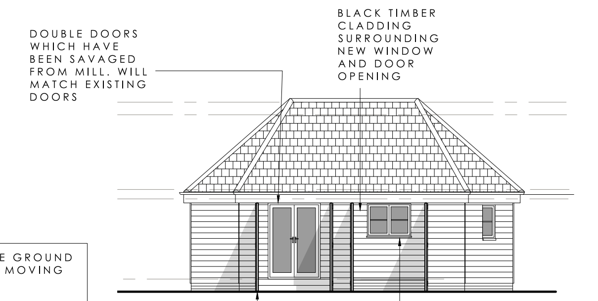
FRONT ELEVATION (DOORS OPEN) PROPOSED 1:100 @ A1
