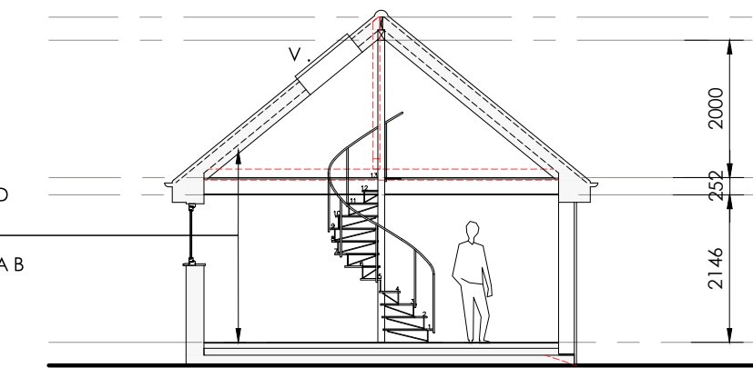
SECTION B-B PROPOSED 1:100 @ A1
