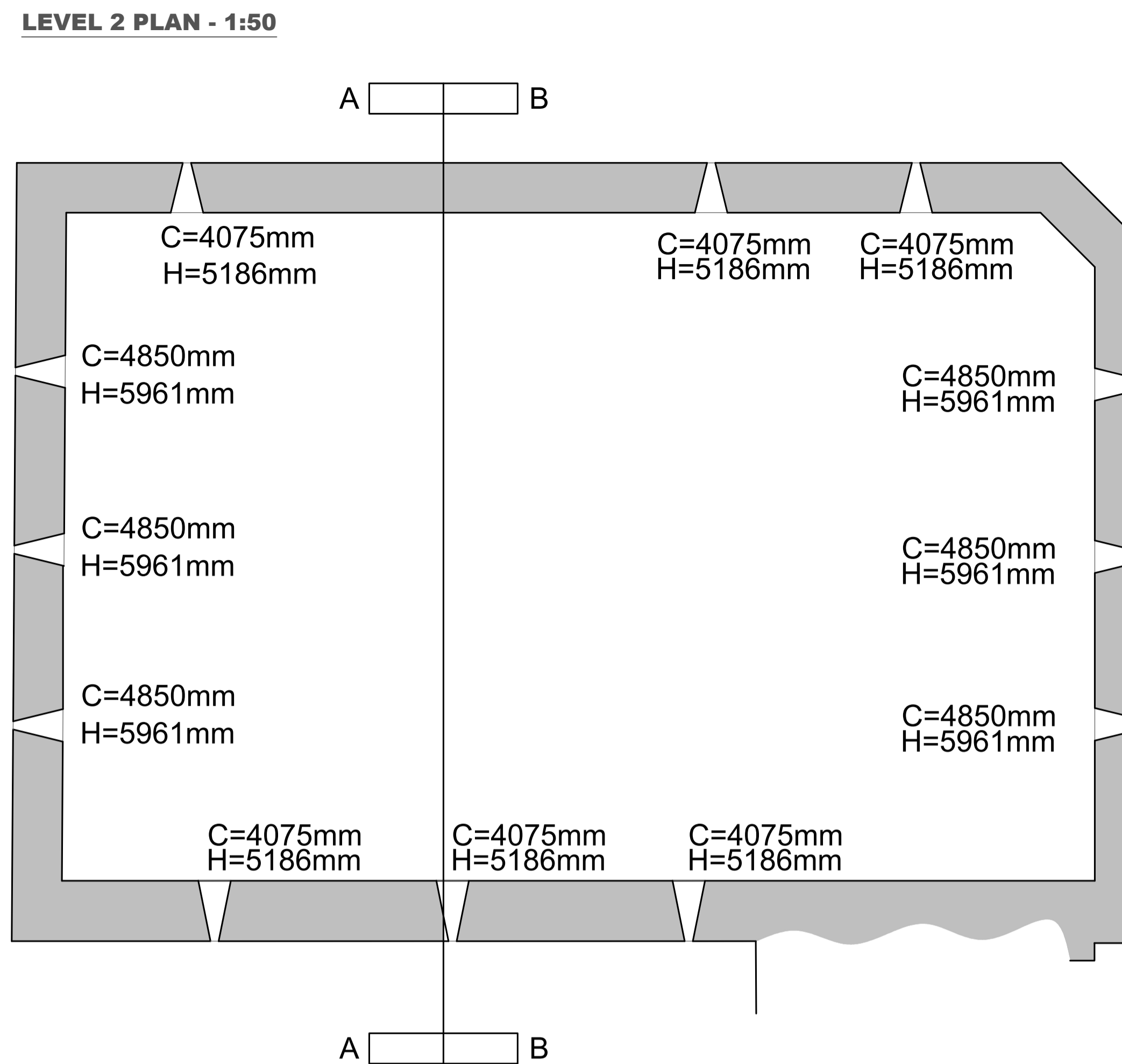
LEVEL 2 PLAN - 1:50
