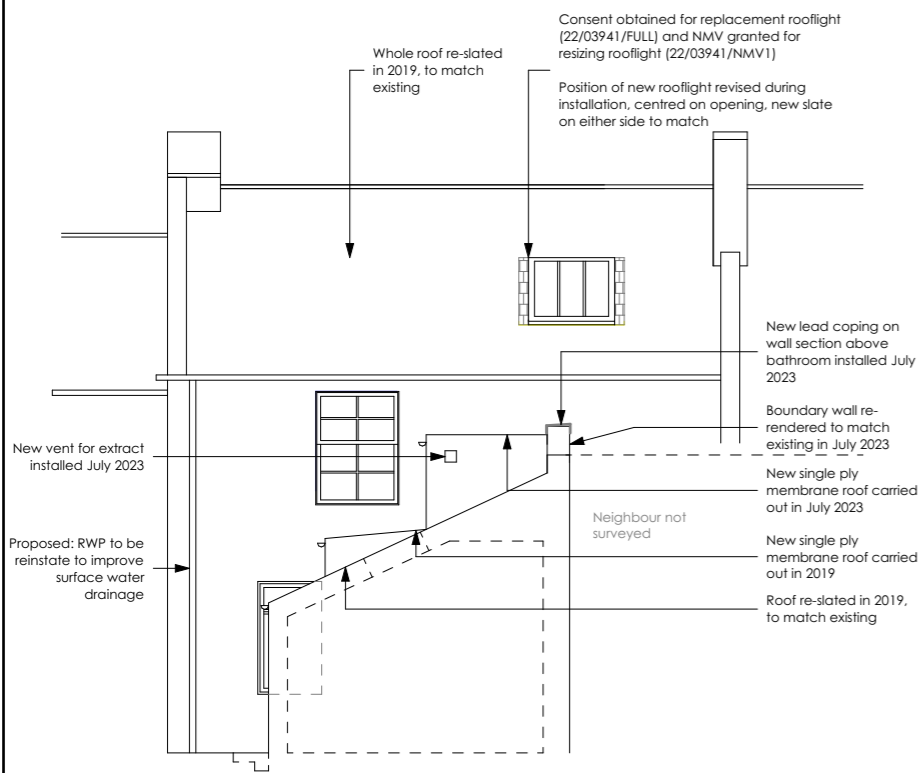
Proposed West Elevation 1:100 @ A3
