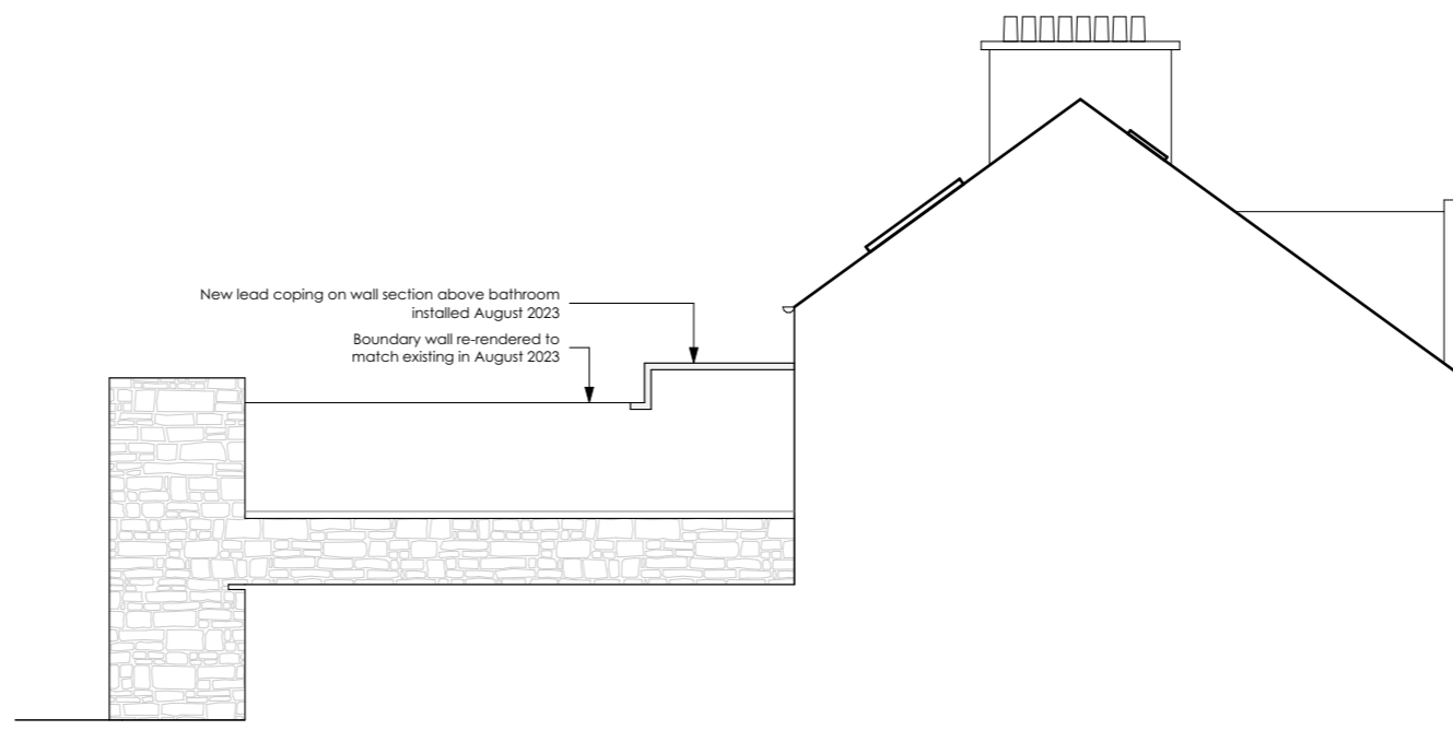
Proposed South Elevation 1:100 @ A3
