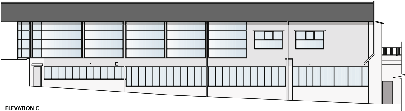
ELEVATION C Proposed Side elevation - scale 1:200 @ A4
