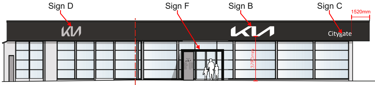
ELEVATION A Proposed Front elevation - scale 1:200 @ A4
