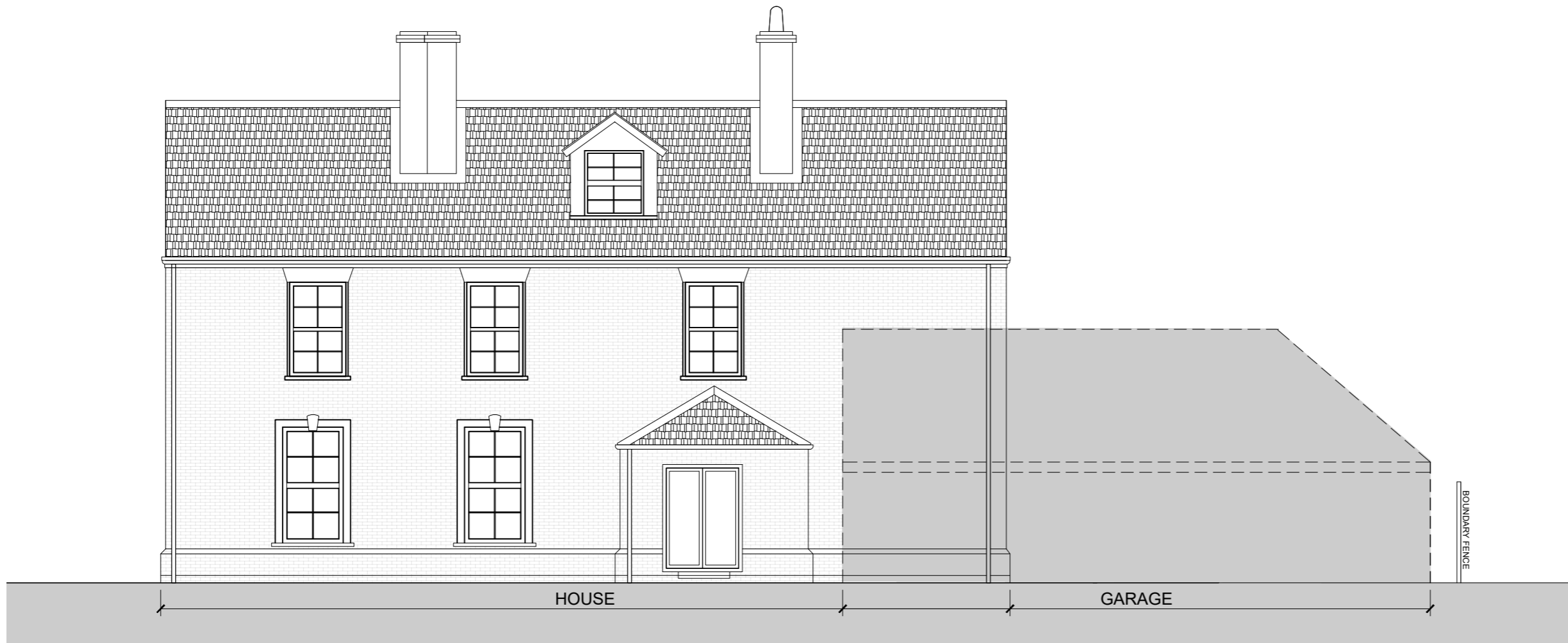
① East Elevation Existing Scale 1:100
