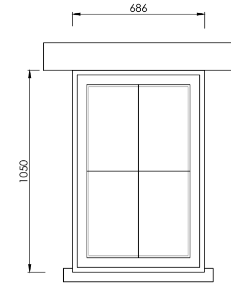
NW-07 & NW-08 - First Floor Window - Double Glazed, Timber Frame
