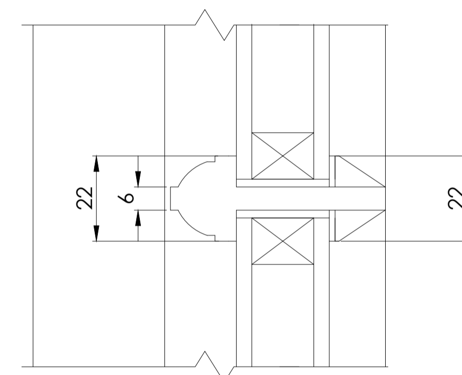
Glazing Bars 1:1
