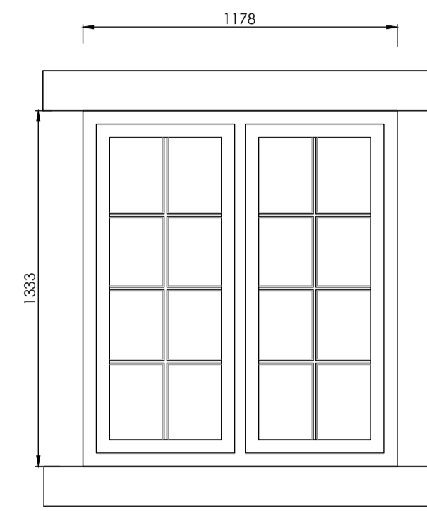
NW-09 - Ground Floor Window - Double Glazed, Timber Frame
