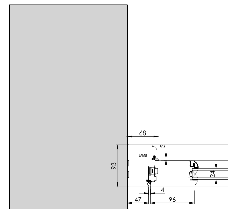
Section A -A 1:5 0 50mm 100mm 150mm 200mm 250mm 300mm 1:5
