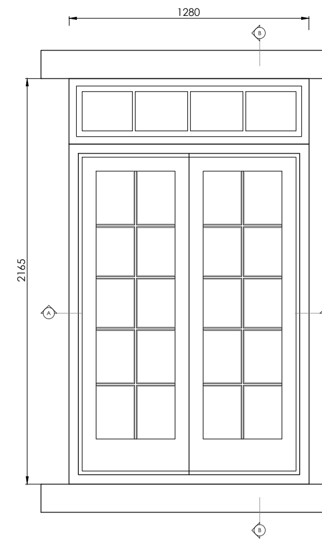
ND-04 - Ground Floor External Door - Double Glazed, Timber Frame by Westbury Windows and joinery.
