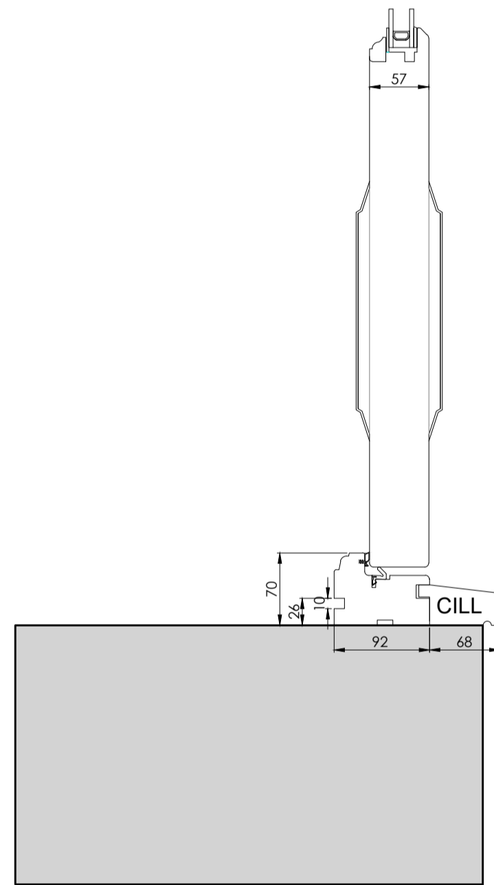
Section B - B 1:5 0 50mm 100mm 150mm 200mm 250mm 300mm 1:5
