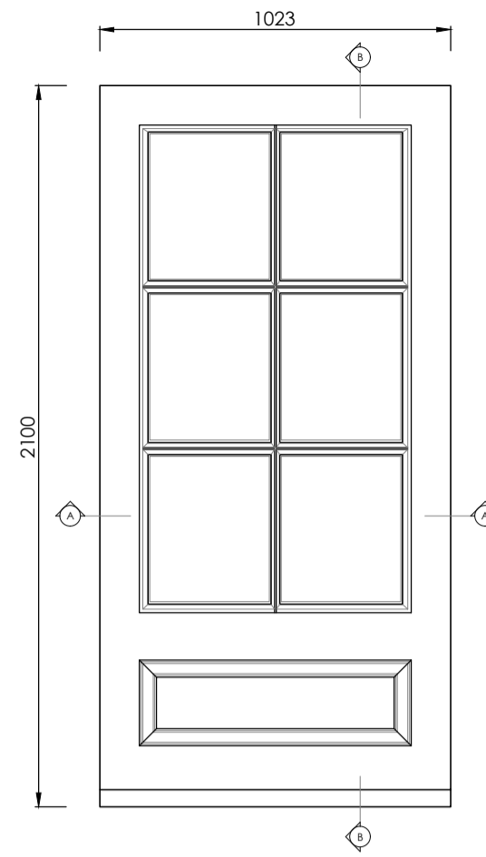
ND-03 - Ground Floor External Door - Double Glazed, Timber Frame by Westbury Windows and joinery.
