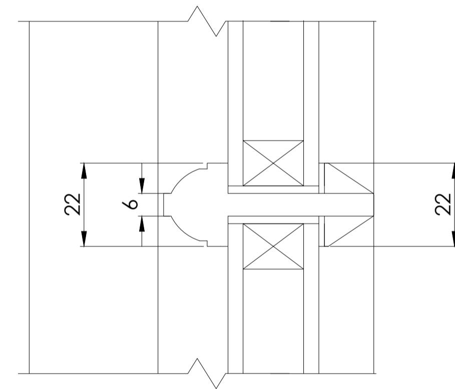
Glazing Bars 1:1 0 10mm 20mm 30mm 40mm 50mm 1:1
