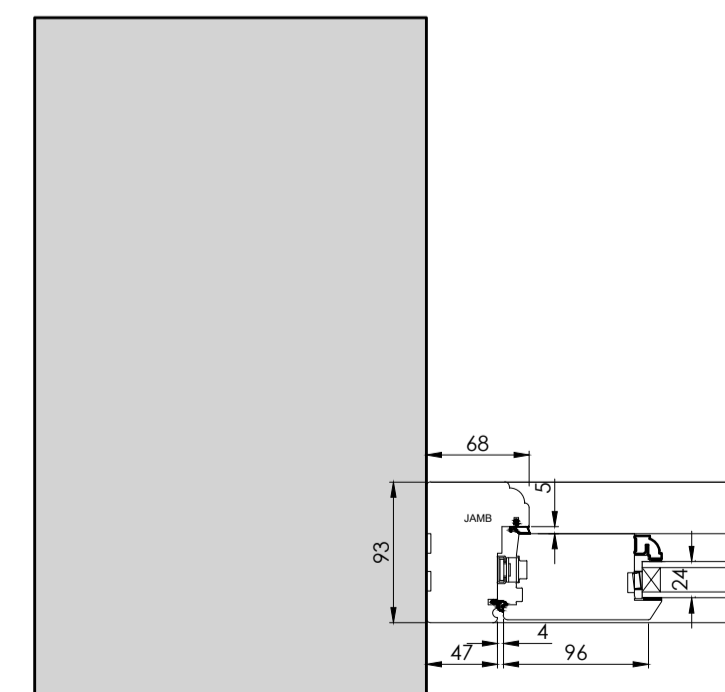
Section A -A 1:5 0 50mm 100mm 150mm 200mm 250mm 300mm 1:5
