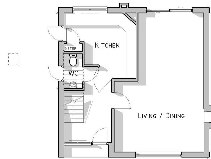
EXISTING GROUND FLOOR PLAN 1 : 100
