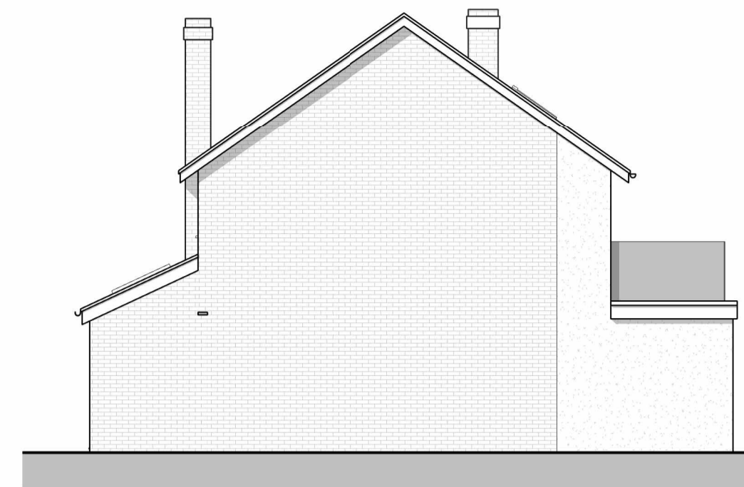
PROPOSED LEFT ELEVATION 1 : 100
