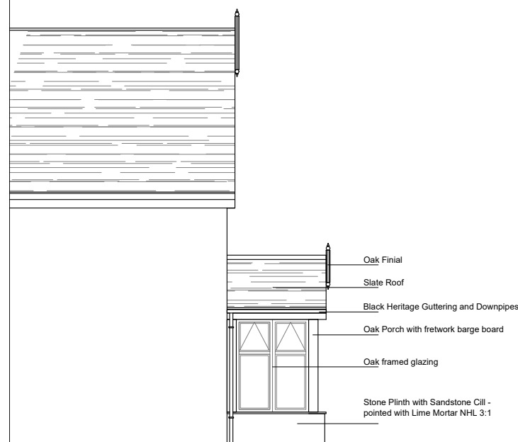
Proposed Front Elevation. North West - (PART)
