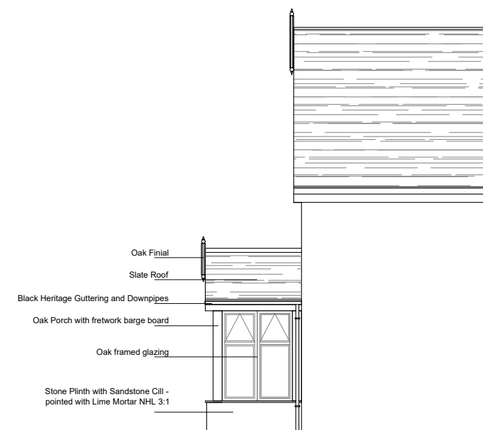
Proposed Rear Elevation. South East - (PART)
