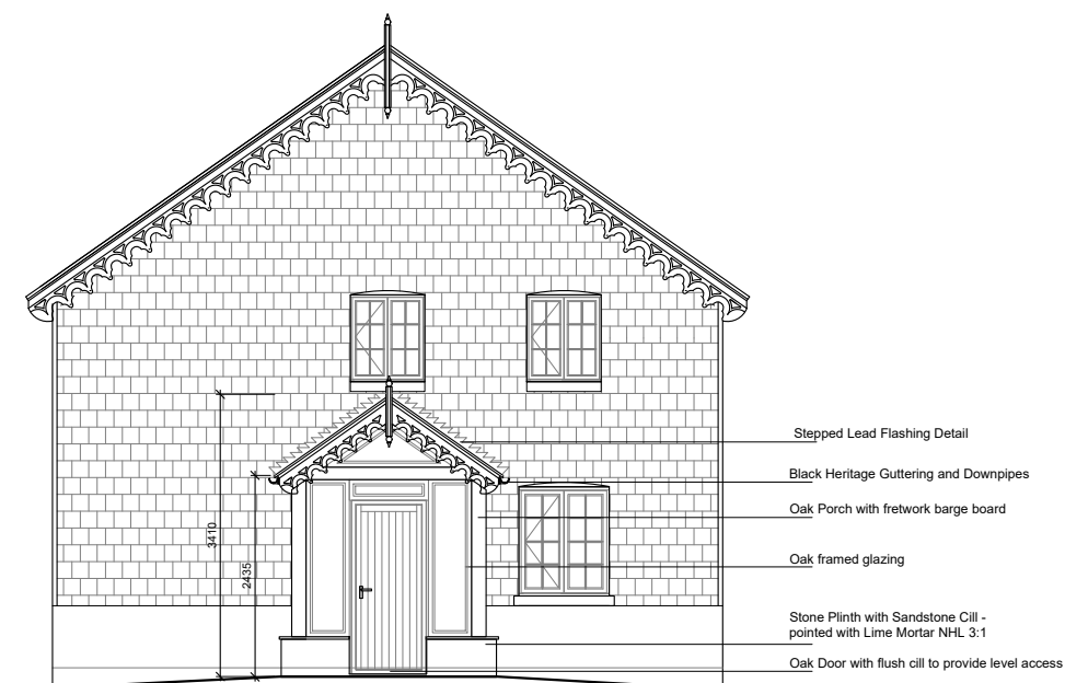
Proposed Side Elevation. South West - (PART)
