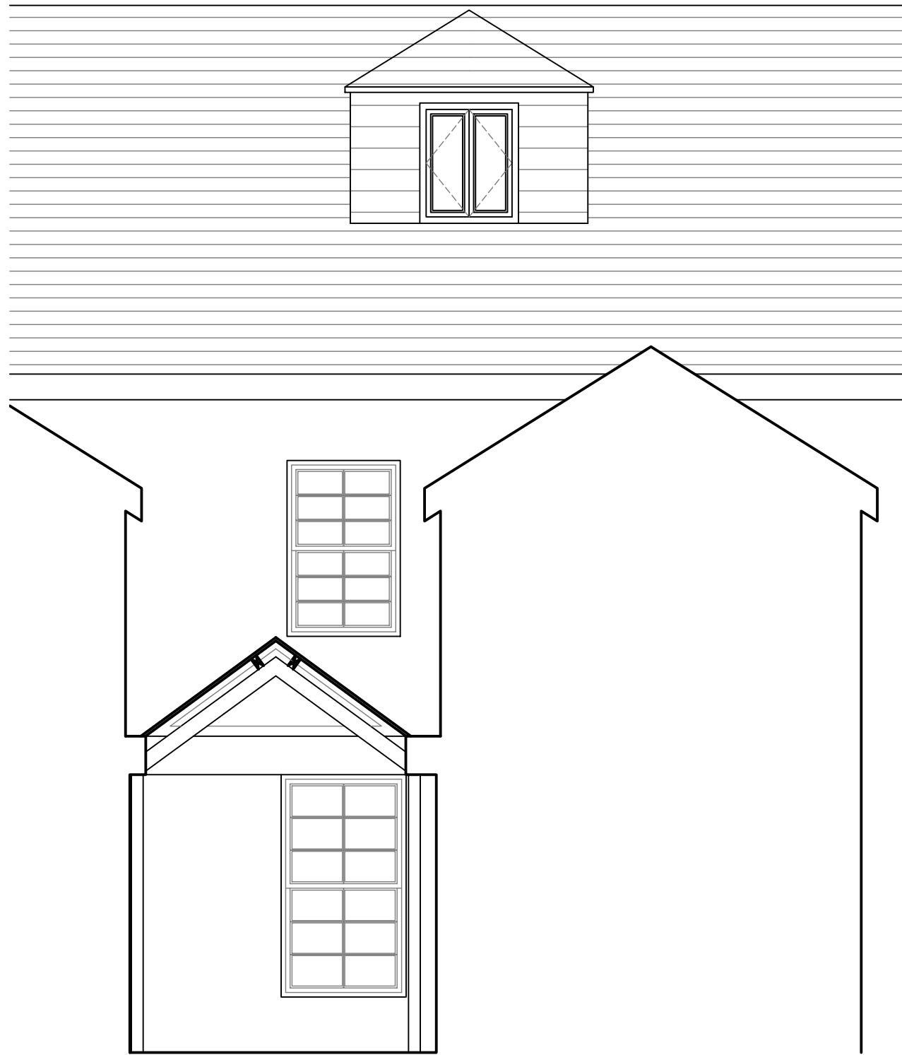
existing NW elevation scale 1:50 @A3
