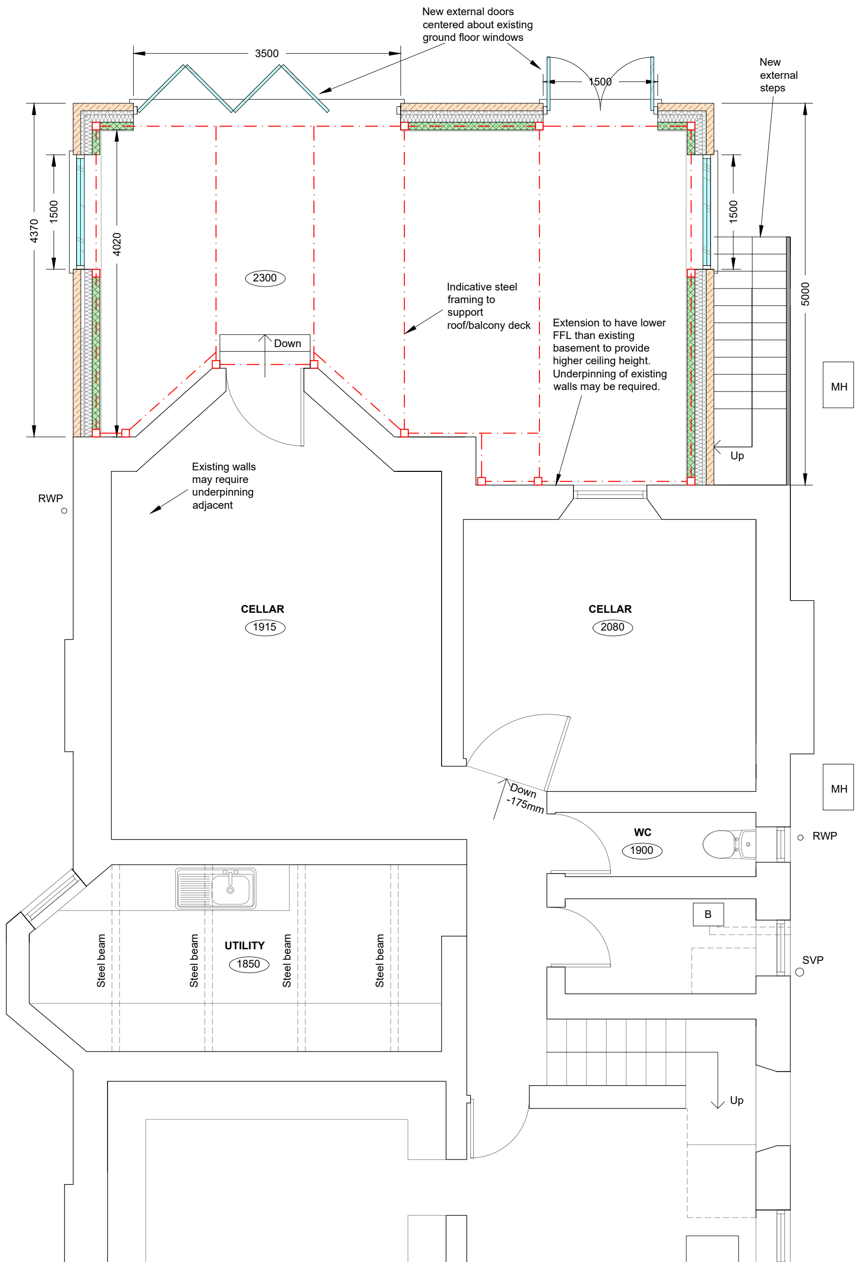
PROPOSED BASEMENT PLAN
