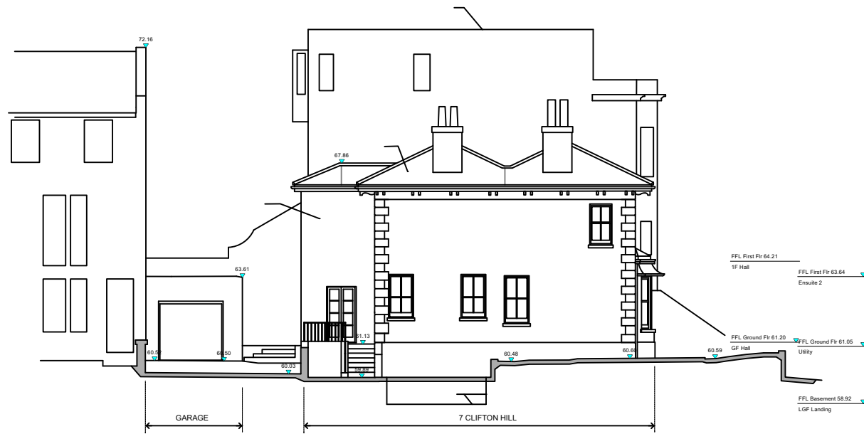
EXISTING NORTH WEST ELEVATION SCALE: 1:200 @A3
