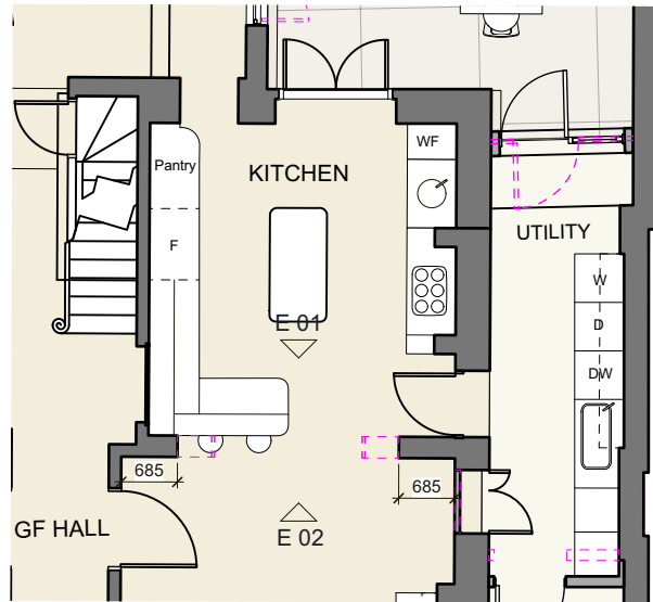
KITCHEN PLAN
