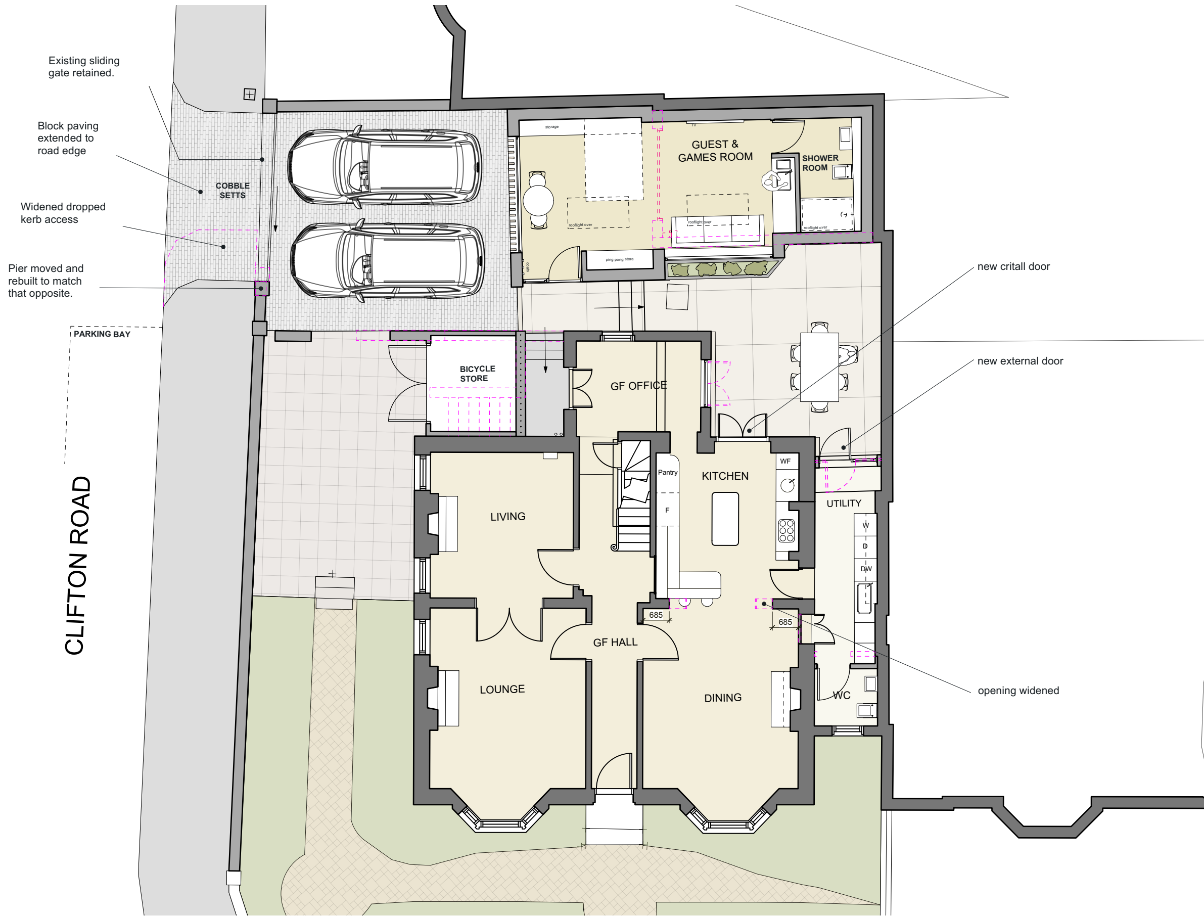
GROUND FLOOR PLAN - PROPOSED SCALE: 1:100 @A3
