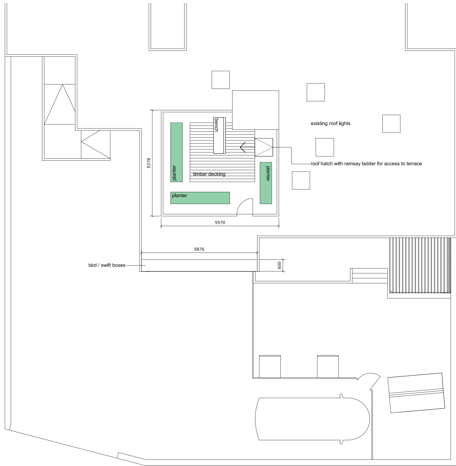
ROOF PLAN
