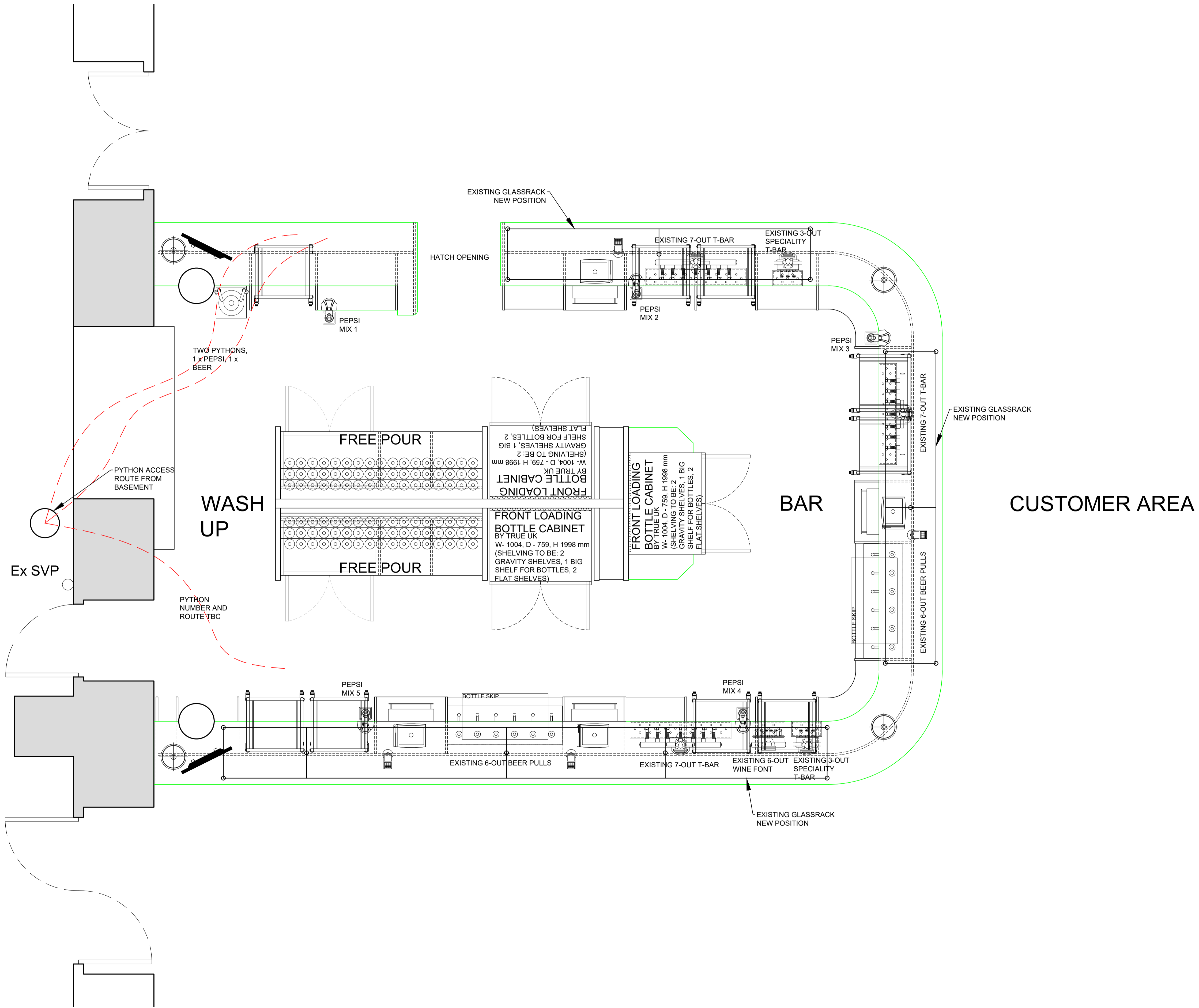
EXISTING BAR PLAN Scale 1:20
