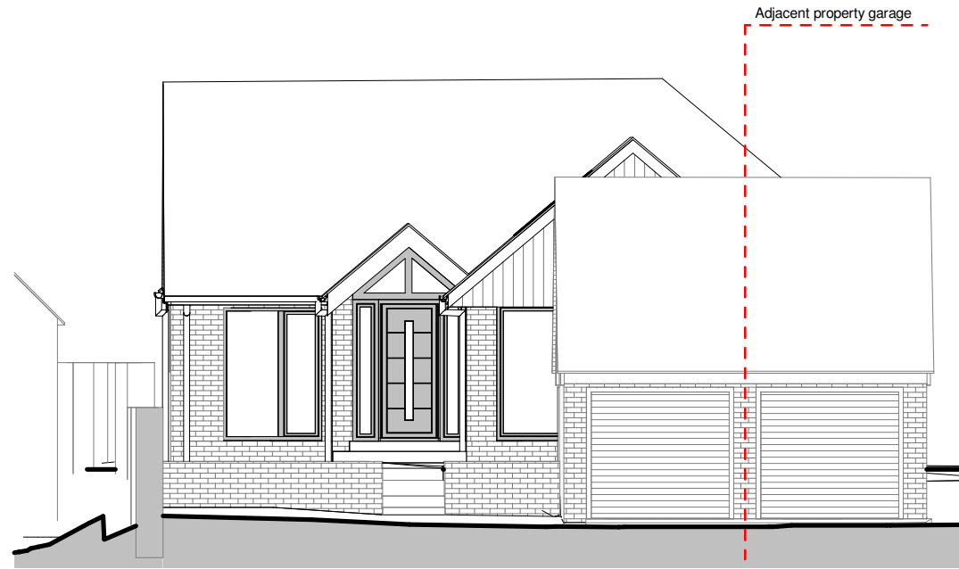
Proposed East Elevation 01
