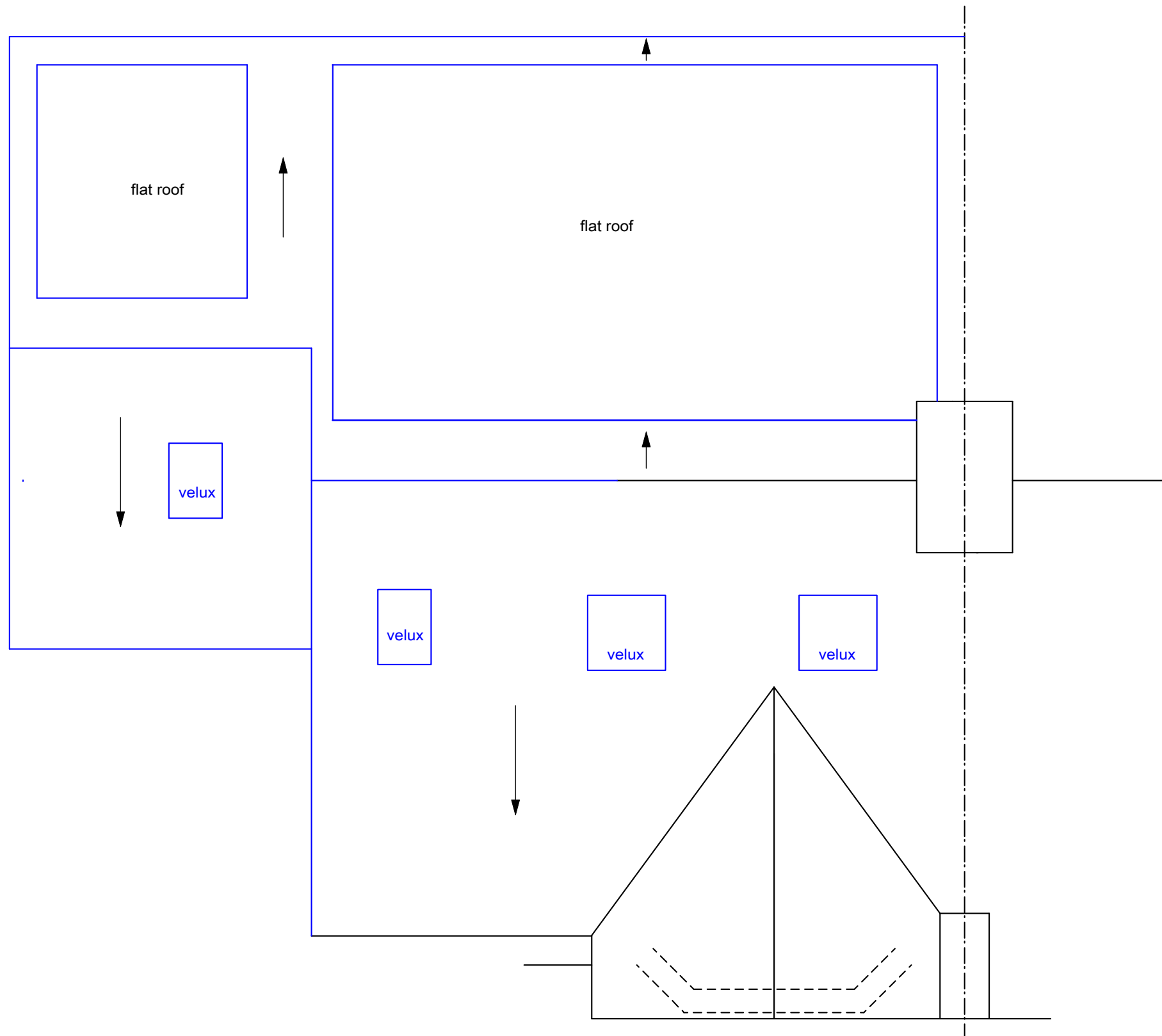
ROOF PLAN
