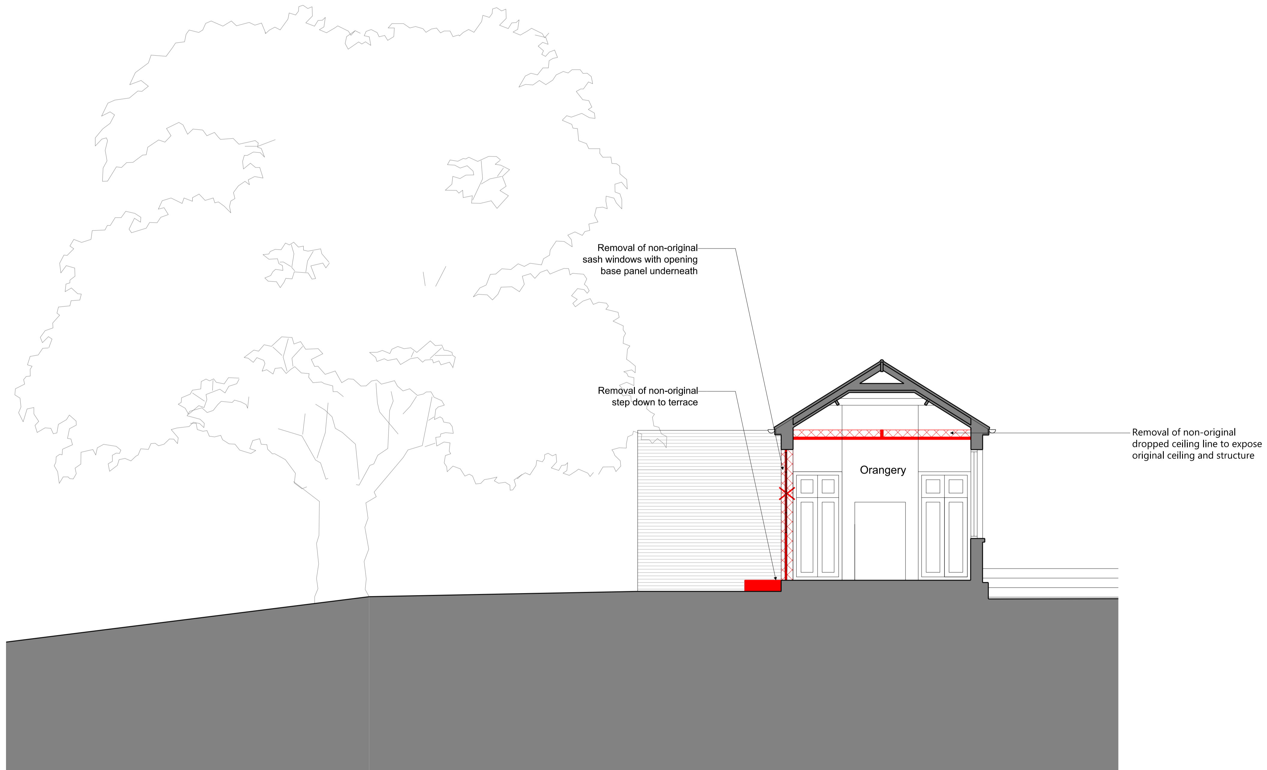
01 Existing: Section BB 1:50 @ A1
