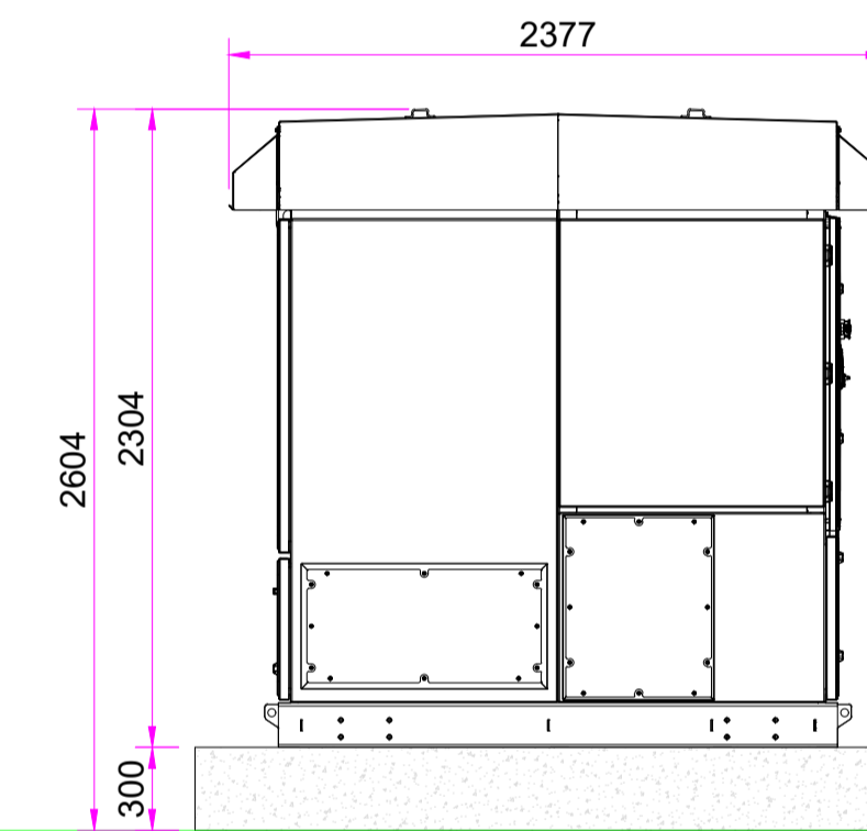
PCS INVERTER – SIDE ELEVATIONS
