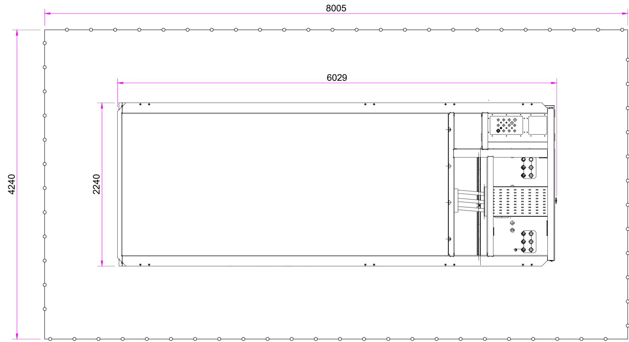
TRANSFORMER / RING MAIN UNIT SKID – PLAN VIEW
