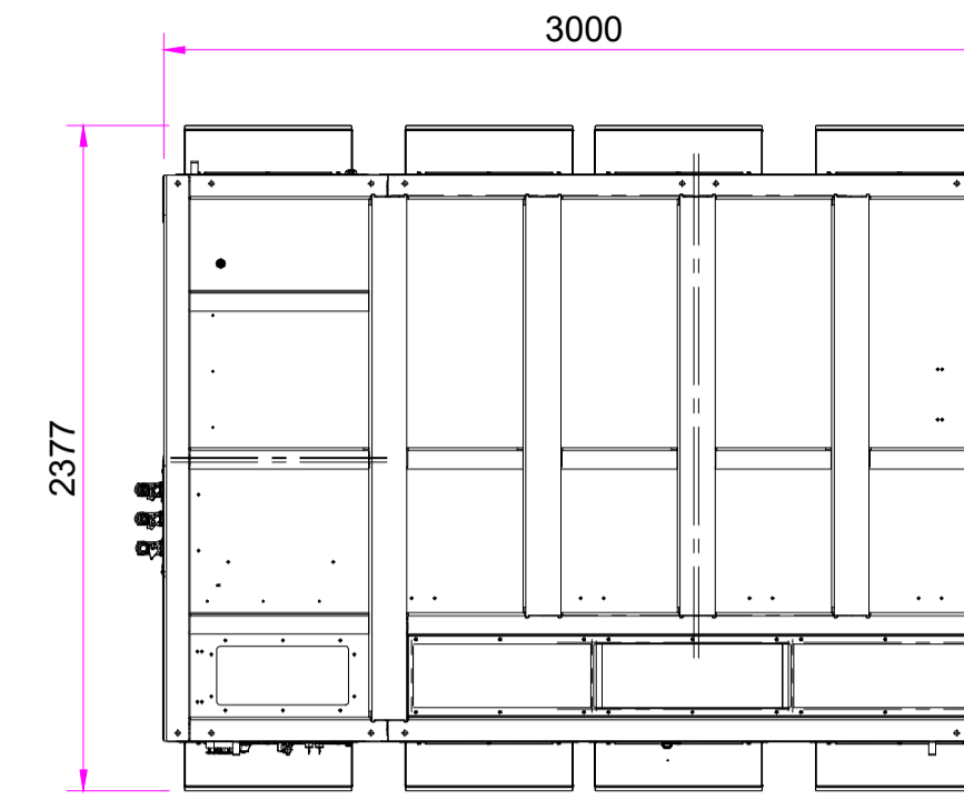
PCS INVERTER – PLAN VIEW
