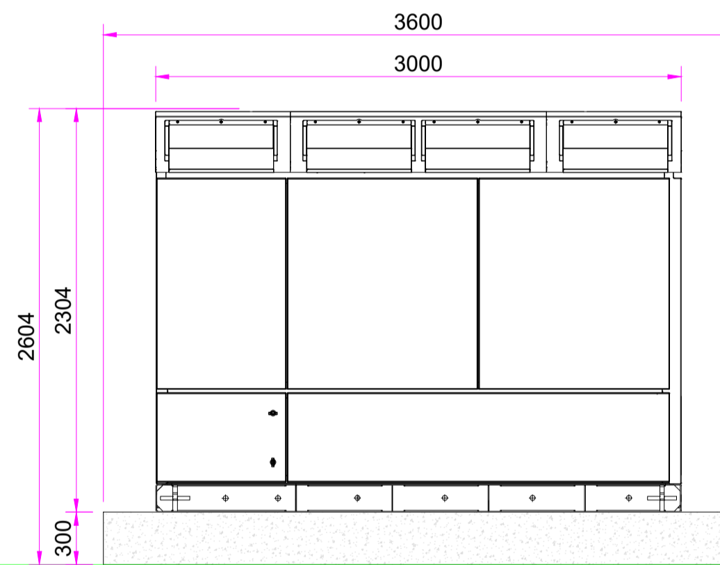
PCS INVERTER – REAR ELEVATION
