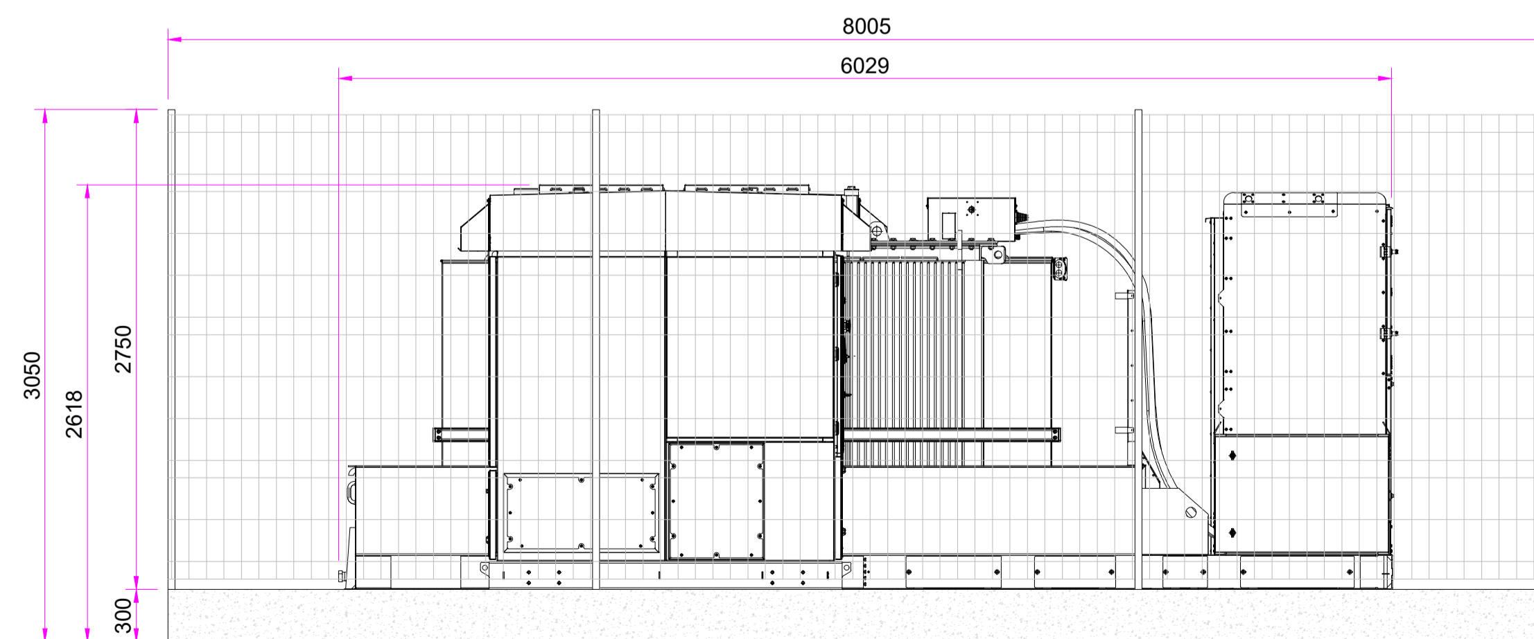
TRANSFORMER / RING MAIN UNIT SKID – FRONT/REAR ELEVATIONS
