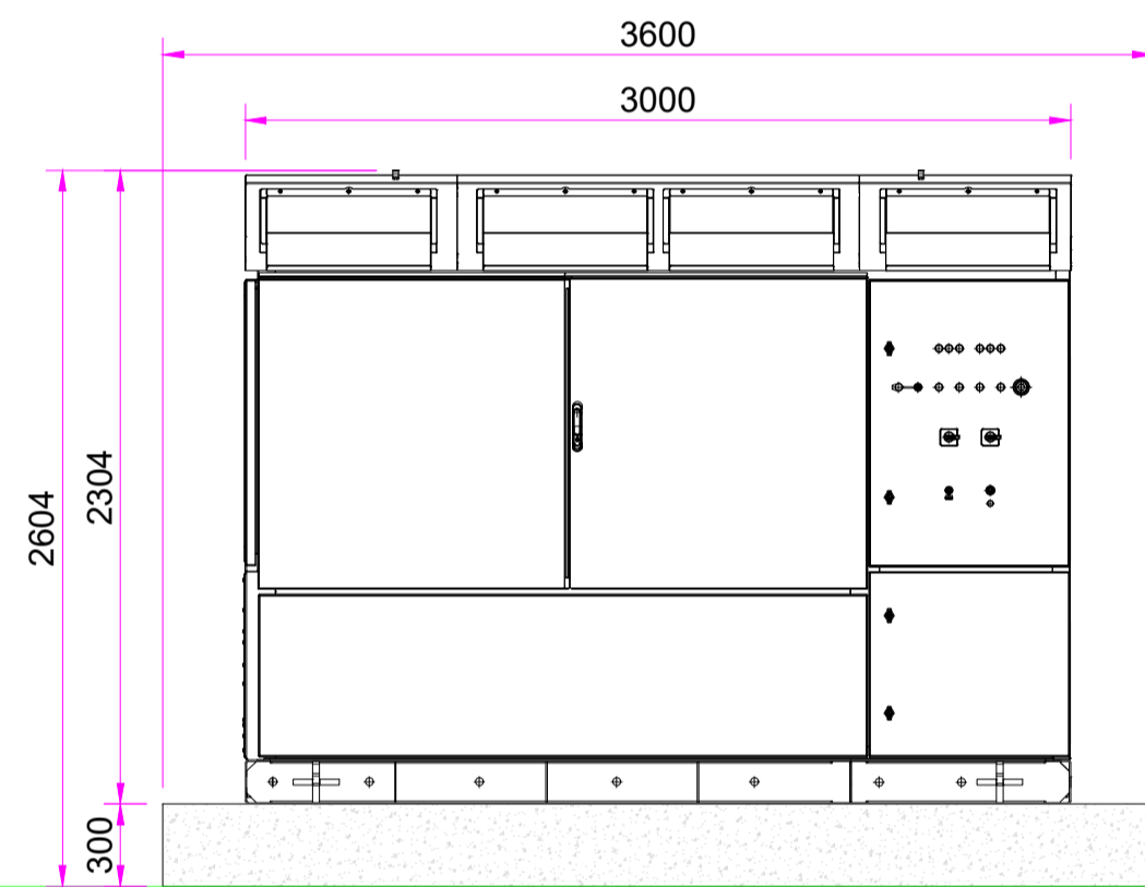
PCS INVERTER – FRONT ELEVATION
