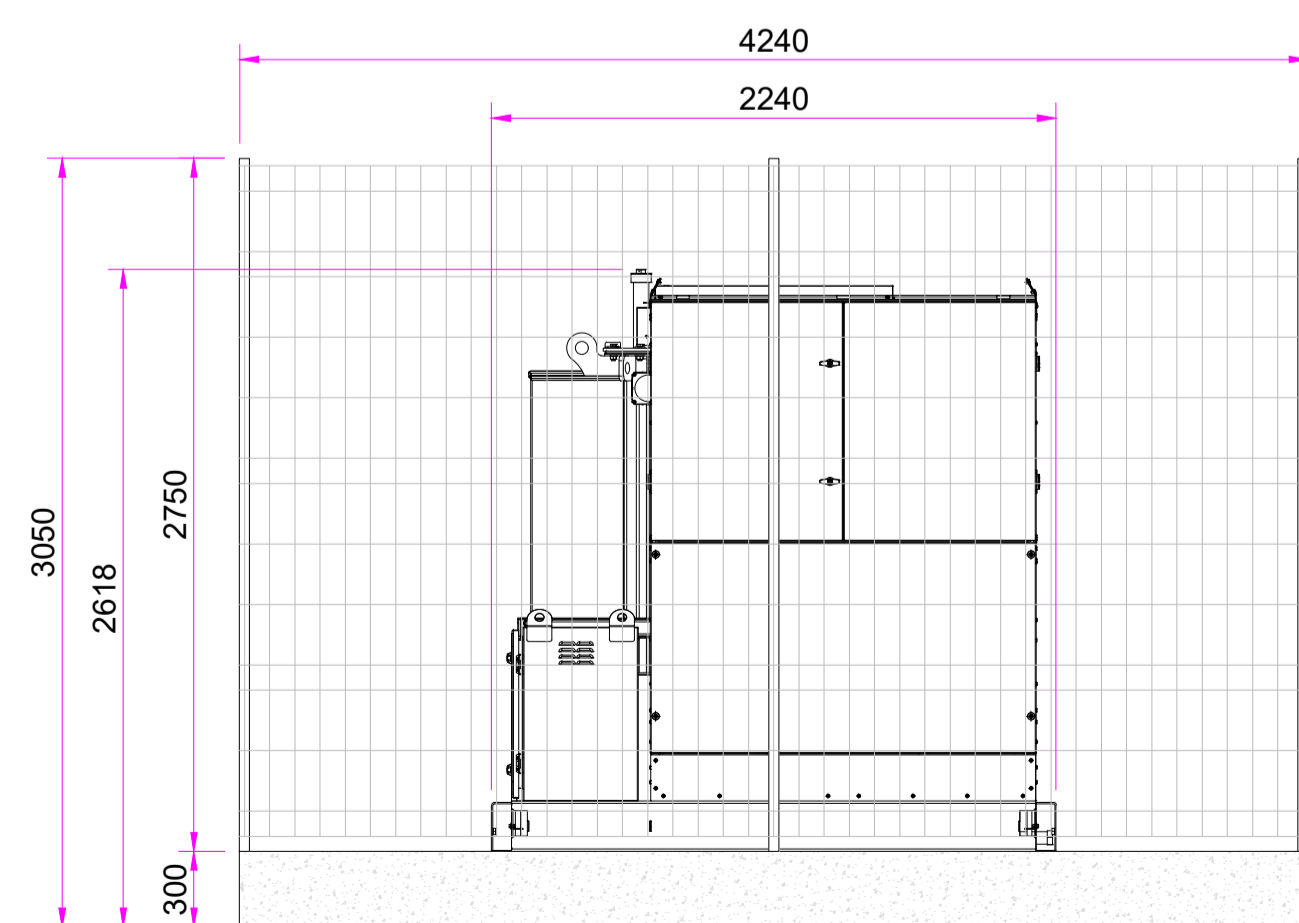
TRANSFORMER / RING MAIN UNIT SKID – SIDE ELEVATIONS
