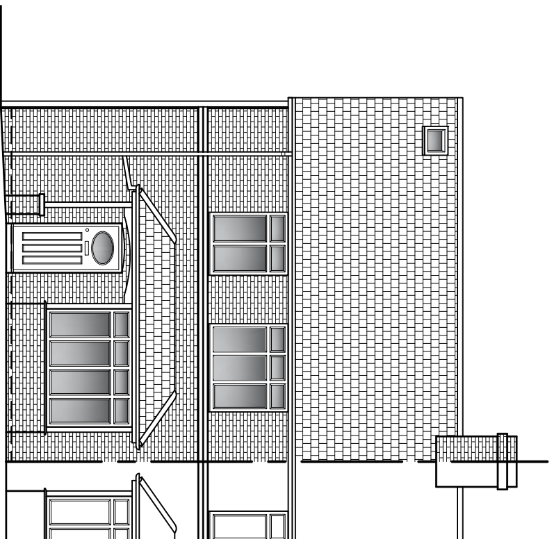
FRONT ELEVATION
