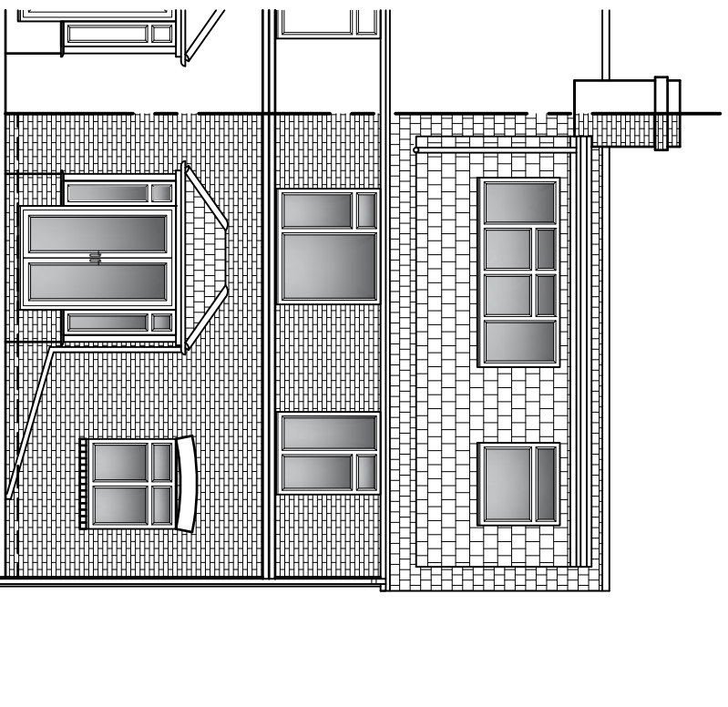
REAR ELEVATION
