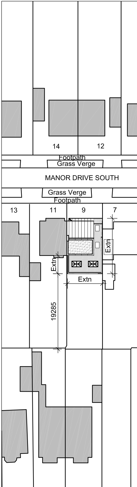
SITE BLOCK PLAN (1:500)
