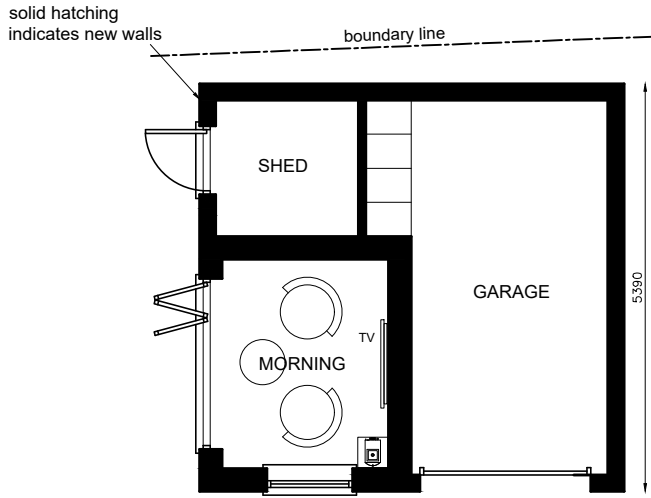
GARAGE / ANNEX PLAN
