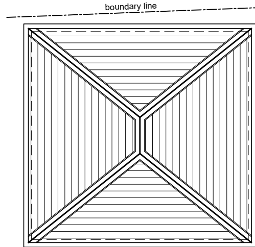
ROOF COVER PLAN
