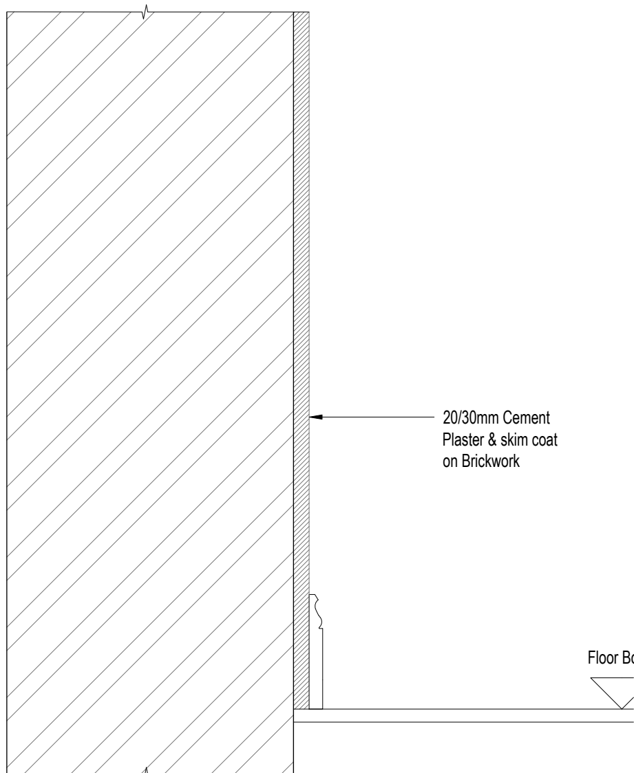
EXISTING SECTION (1:100)
