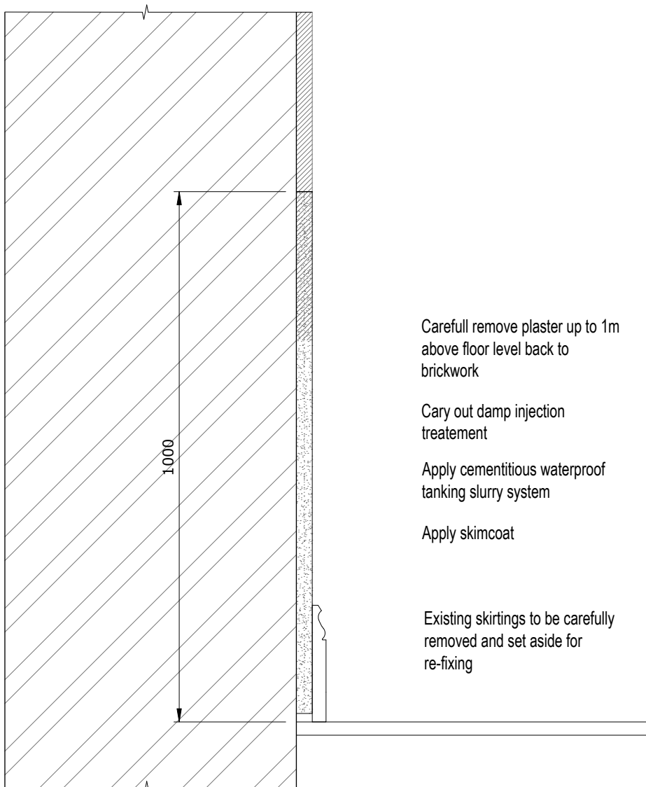
PROPOSED SECTION (1:100)
