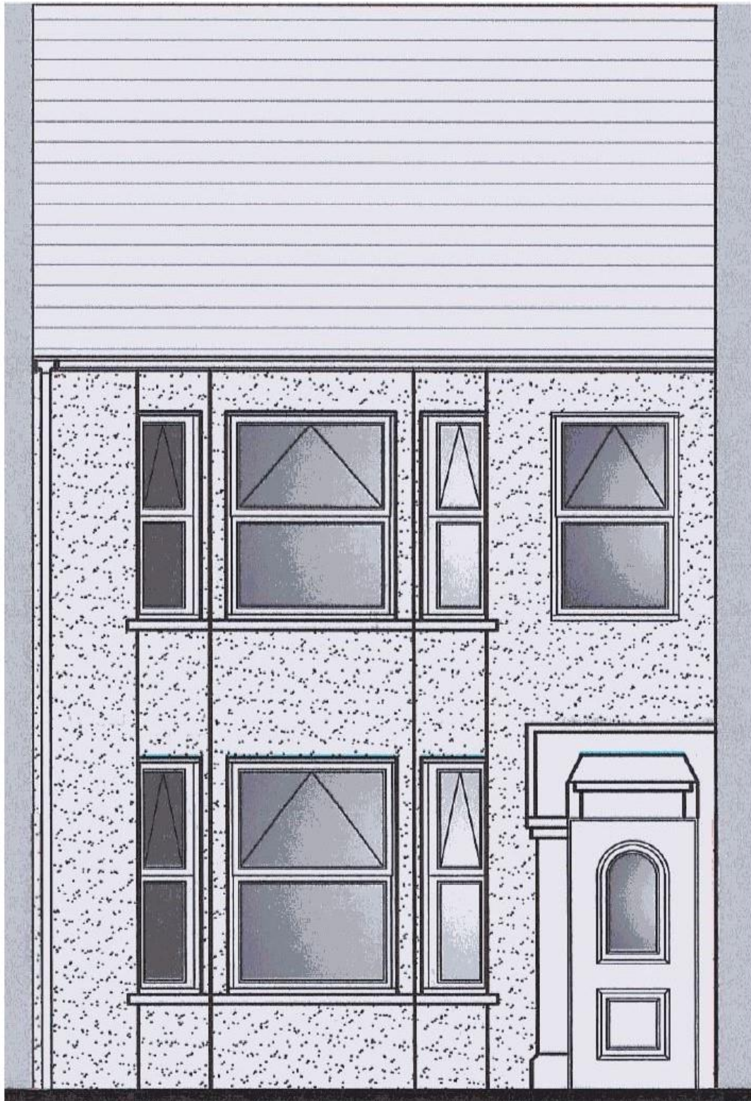
Front Elavation
