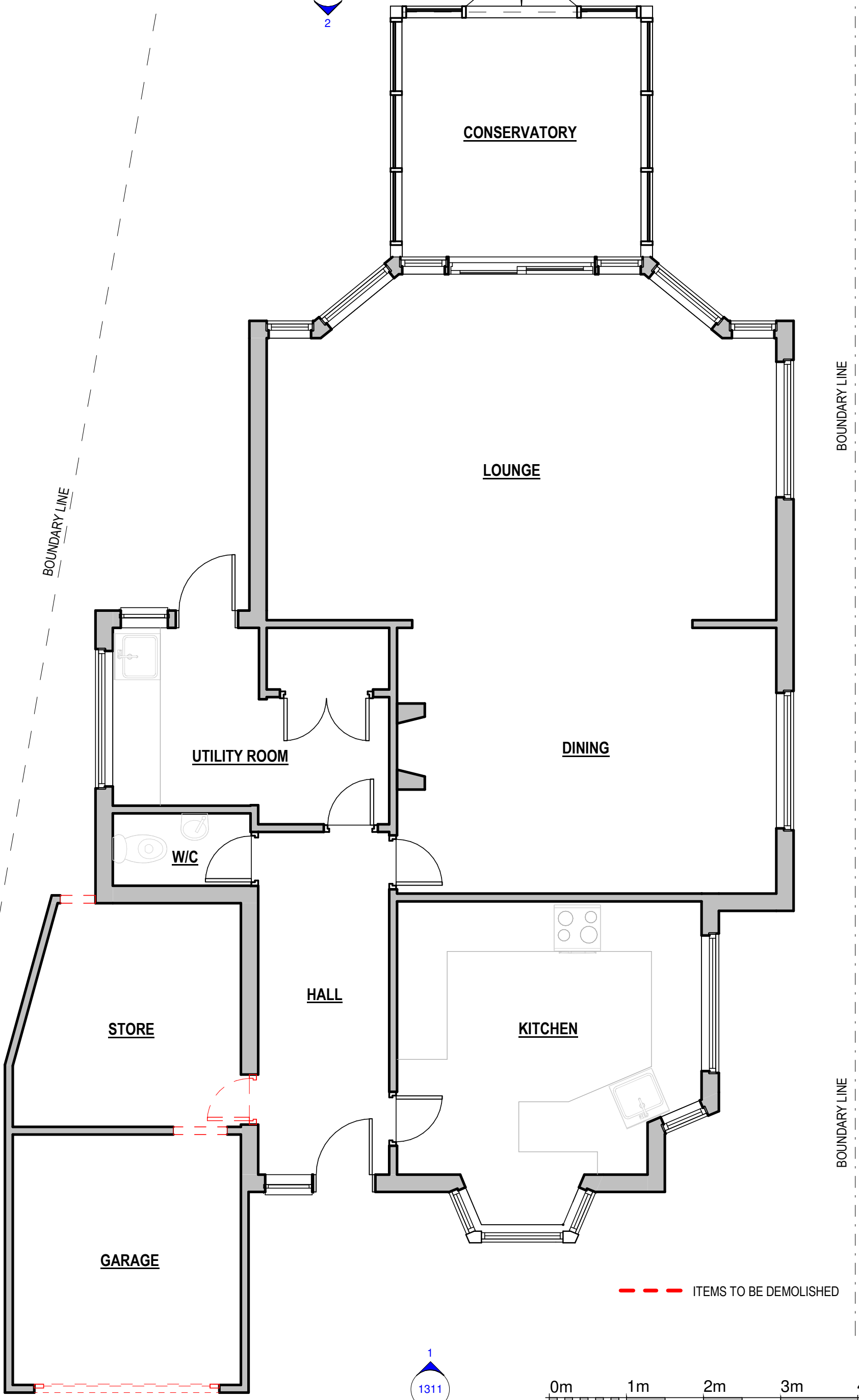
Existing - 00 Ground Floor Plan
