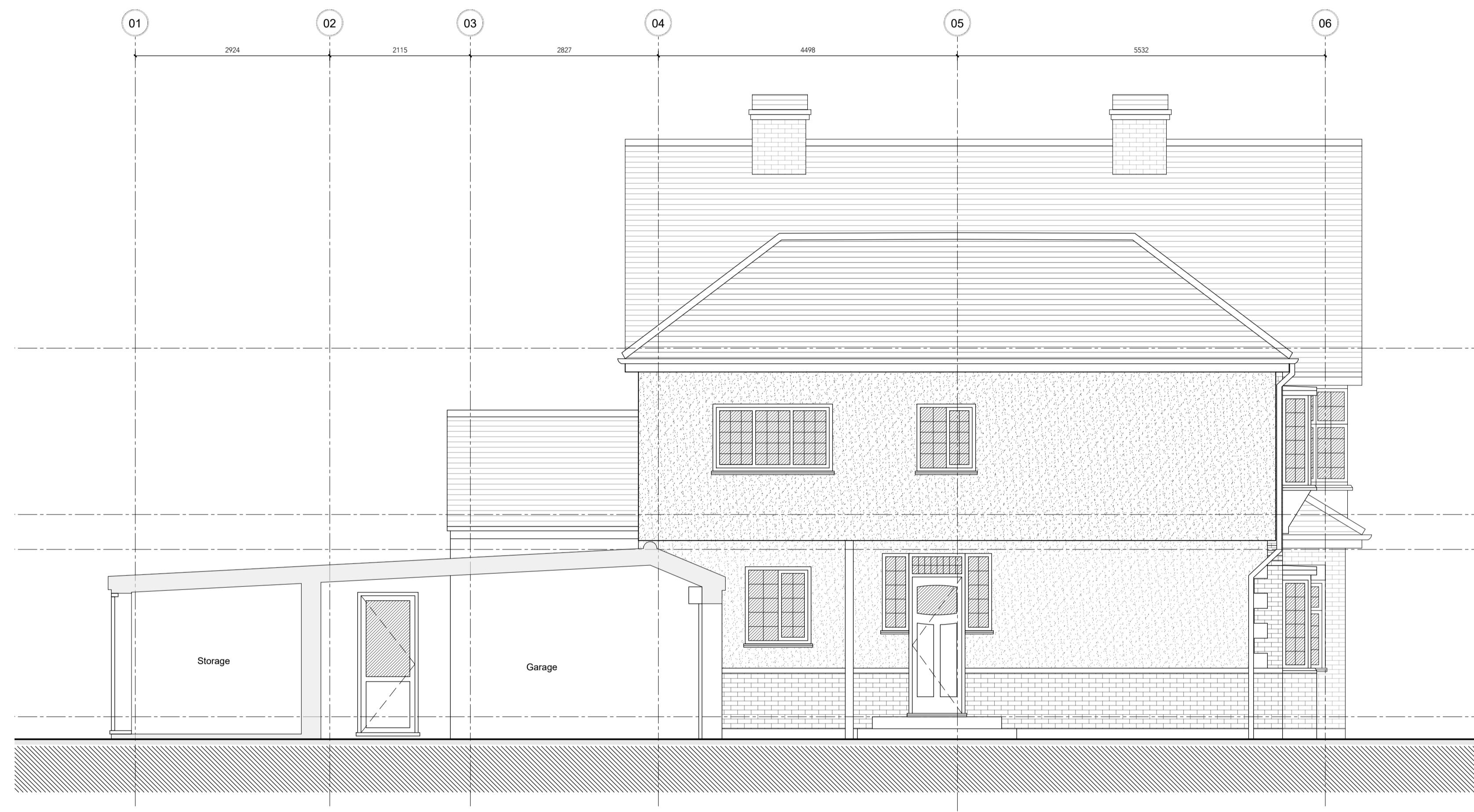
EXISTING: SIDE ELEVATION 03 Scale 1:50
