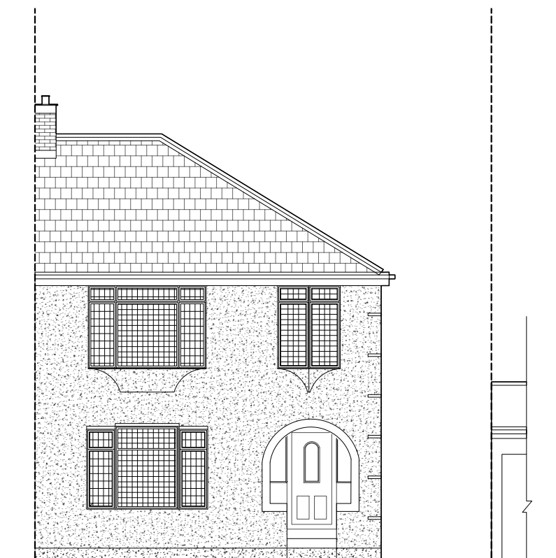
FRONT ELEVATION
