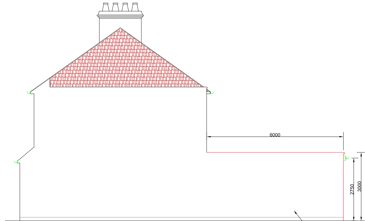
PROPOSED RIGHT SIDE VIEW
