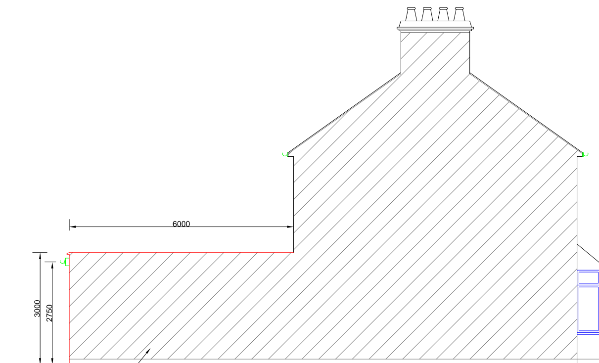
PROPOSED LEFT SIDE VIEW
