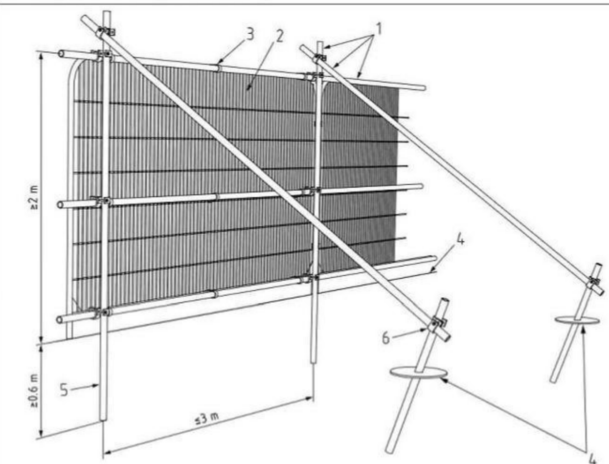
Default specification for protective fencing
