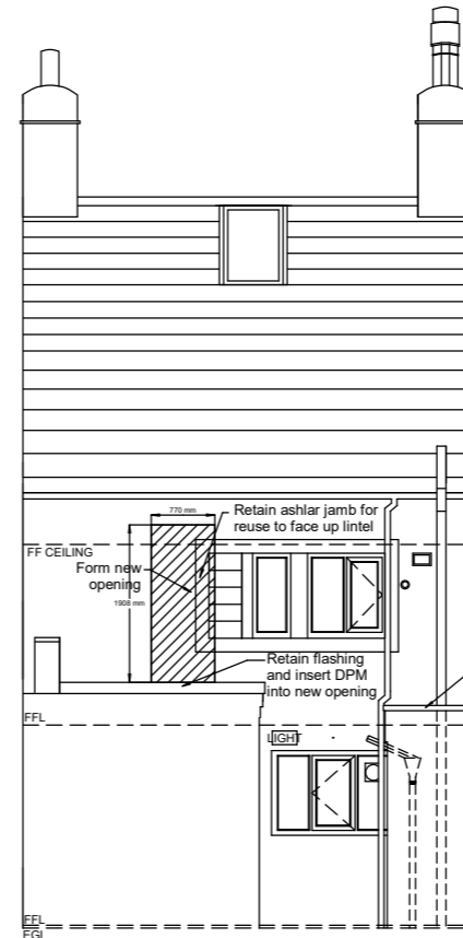
REAR ELEVATION AS EXISTING
