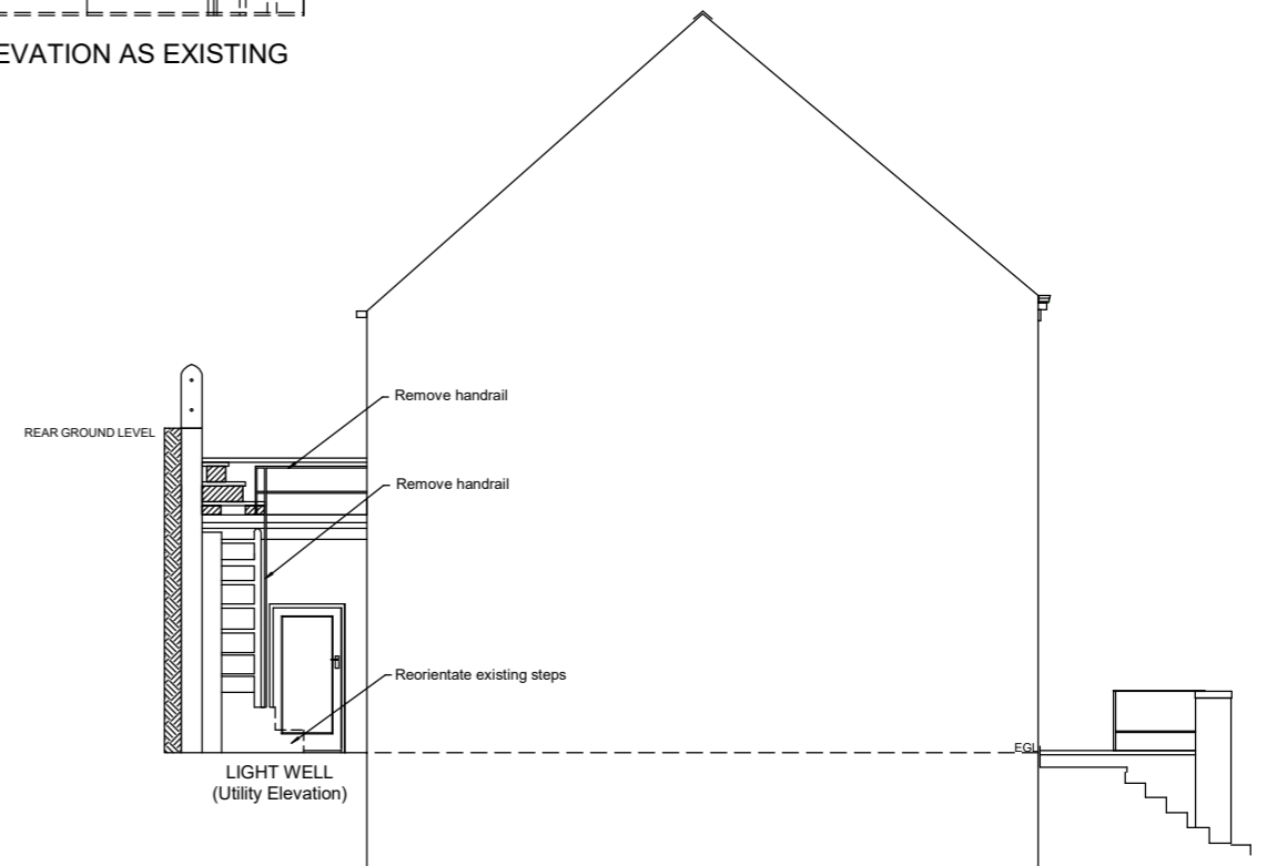
UPPER SIDE ELEVATION AS EXISTING
