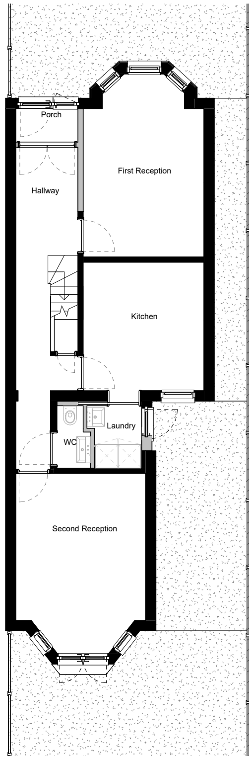
01 Ground Floor Plan - Proposed 1 : 100
