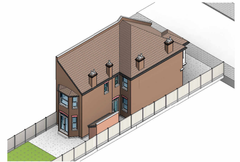
04 3D View - Axonometric Rear - Existing
