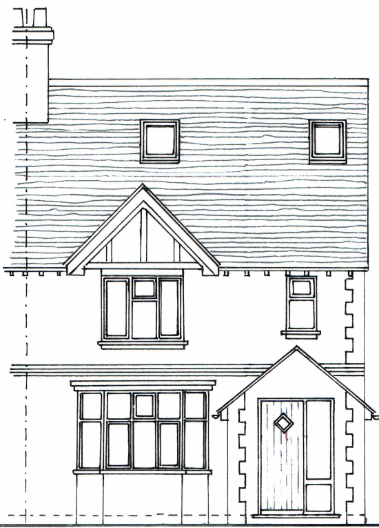
SOUTHEAST ELEVATION
